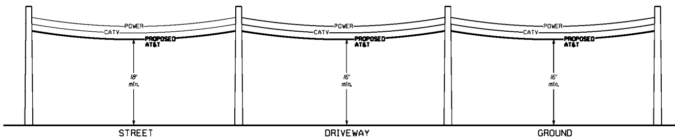
Typical Aerial Clearance Detail
