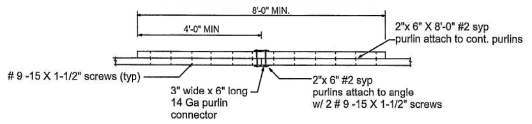
PURLIN CONNECTION TOP VIEW DETAIL
