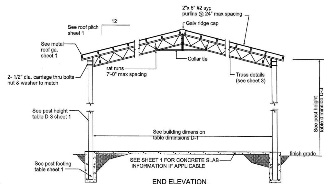
END ELEVATION NTS
