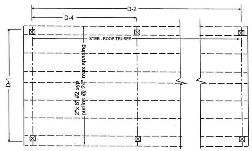
PLAN VIEW POST SPACING
