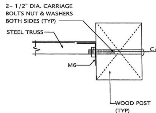
TRUSS TO POST DETAIL PLAN VIEW
