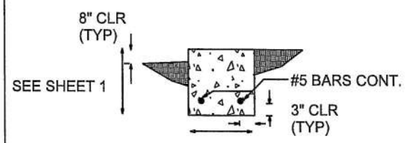
RIBBON FOOTING
