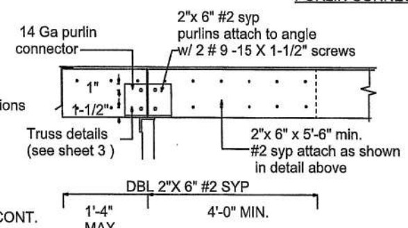
PURLIN TO CONNECTOR GABLE END DETAIL
