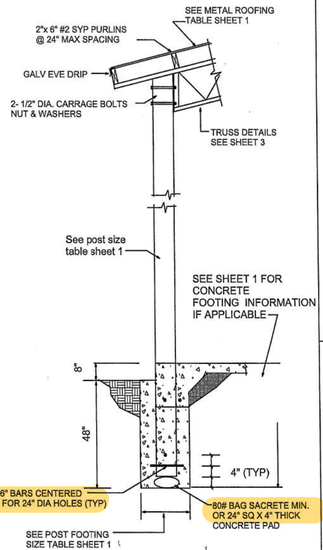
POST FOOTING TO TRUSS DETAIL 1
