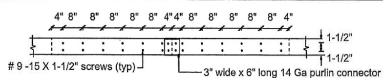
PURLIN CONNECTION SIDE VIEW DETAIL
