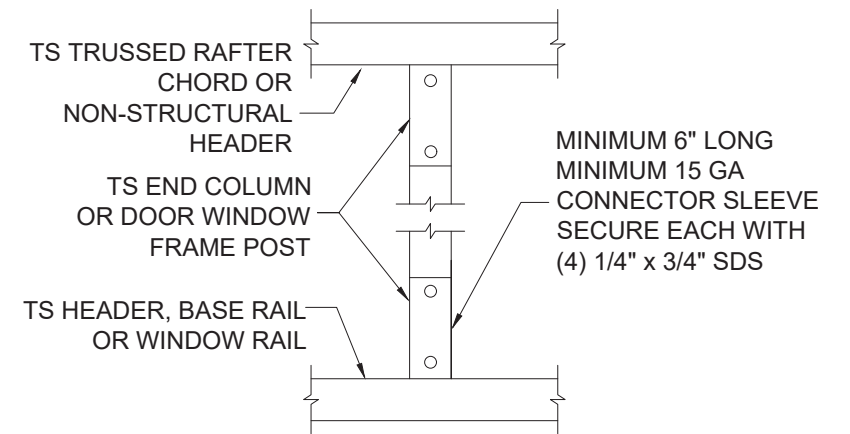
10 POST TO HEADER, BASE RAIL CONNECTION SCALE: NTS
