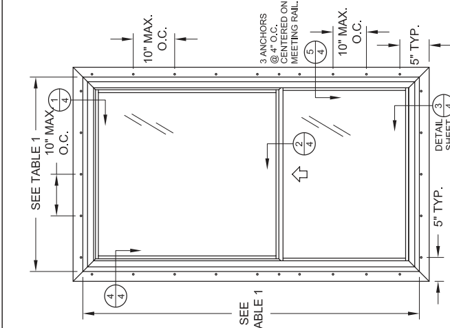
TYP. FIN ANCHOR LOCATIONS (B) (INTEGRAL FIN FRAME, MAX. SIZE ORIEL CONFIG.)
