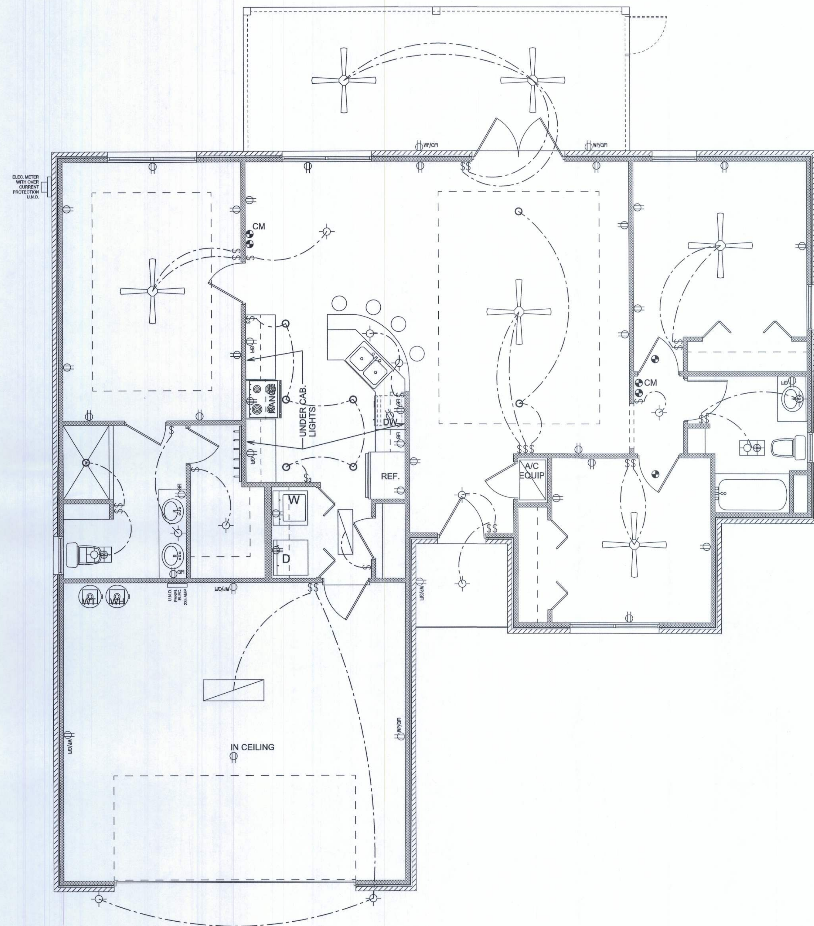
* ELECTRICAL PLAN *
