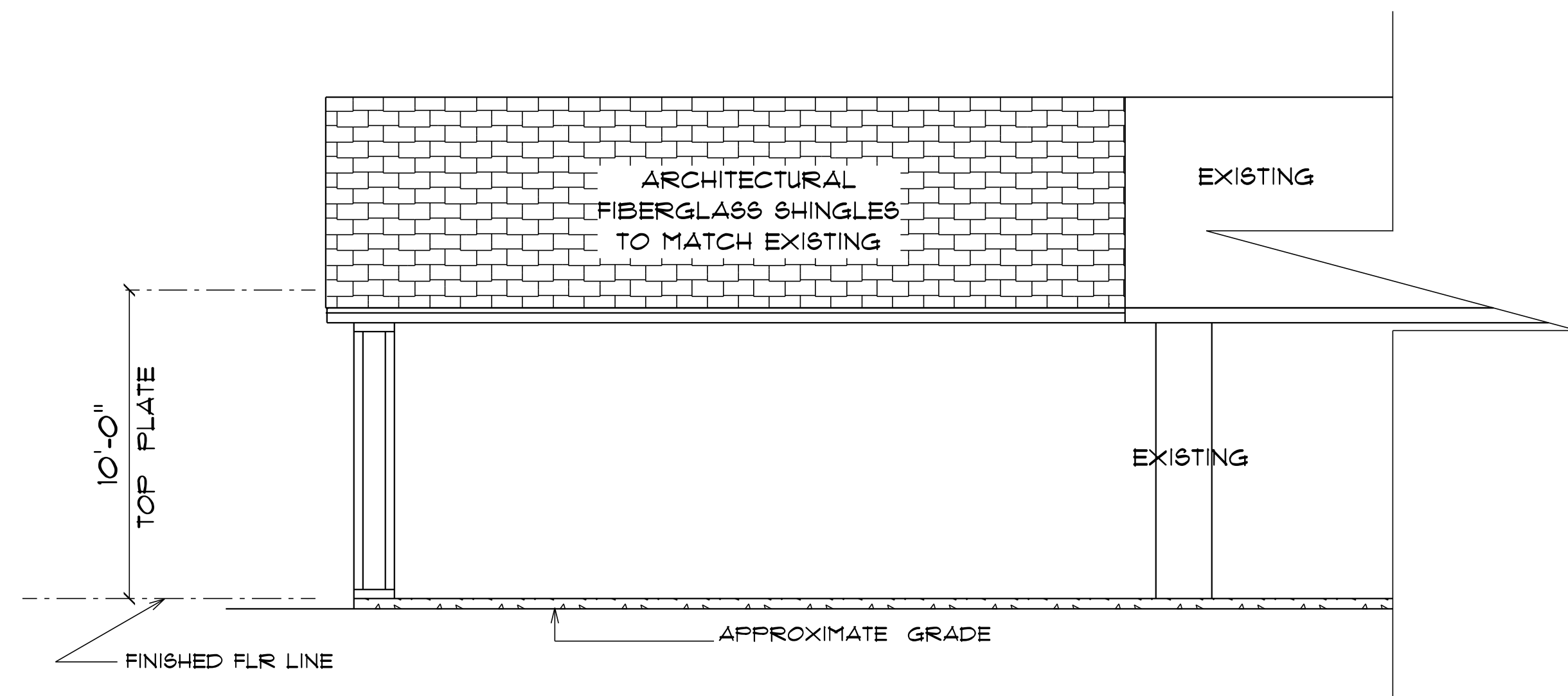
* COVERED PORCH * * LEFT ELEVATION * SCALE : 1/4" = 1'-0"
