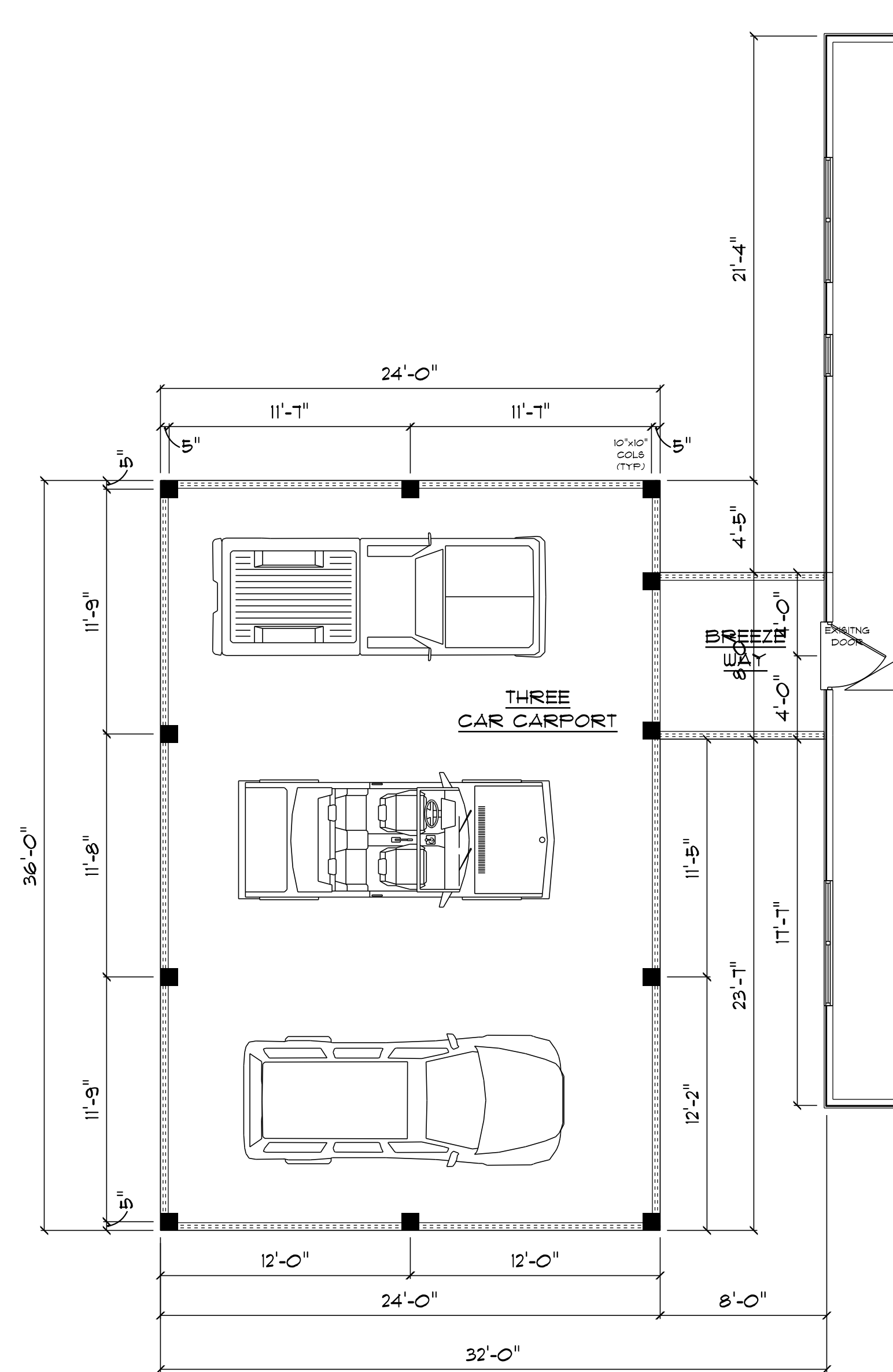
* CARPORT * * FLOOR PLAN * SCALE : 3/16" = 1'-0"
