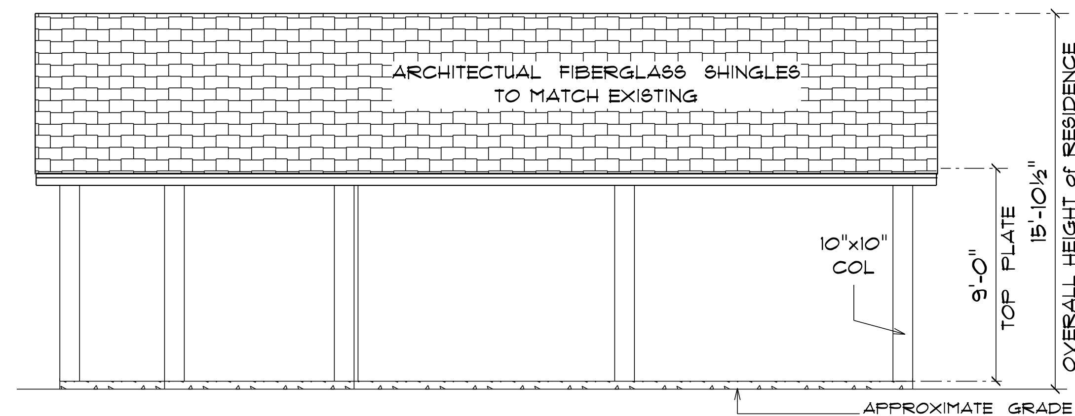
* CARPORT * * LEFT SIDE ELEVATION * SCALE : 1/4" = 1'-0"
