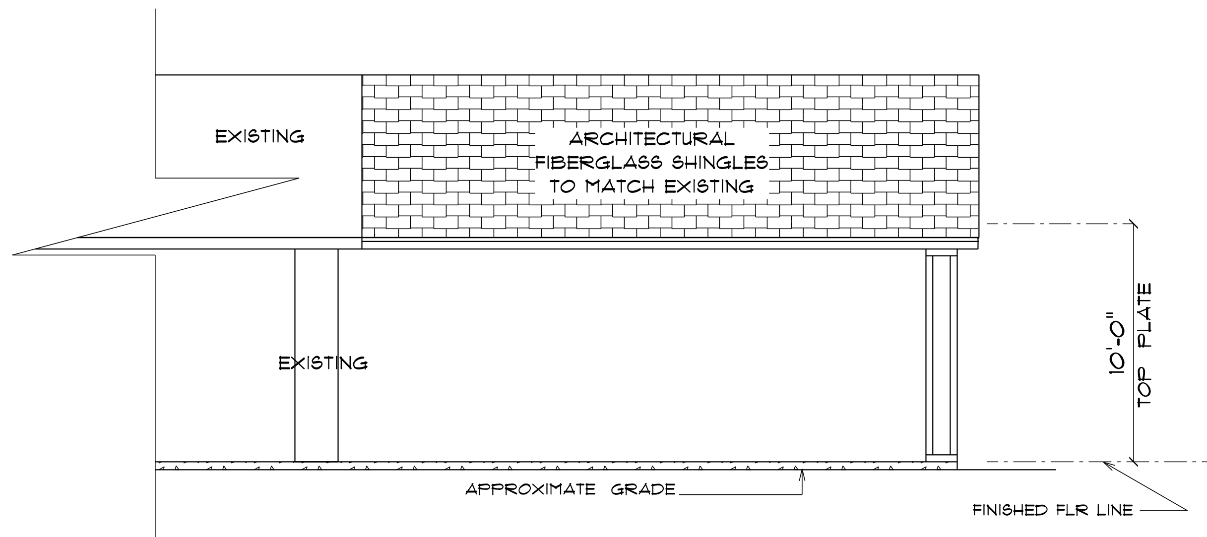
* COVERED PORCH * * RIGHT ELEVATION * SCALE : 1/4" = 1'-0"
