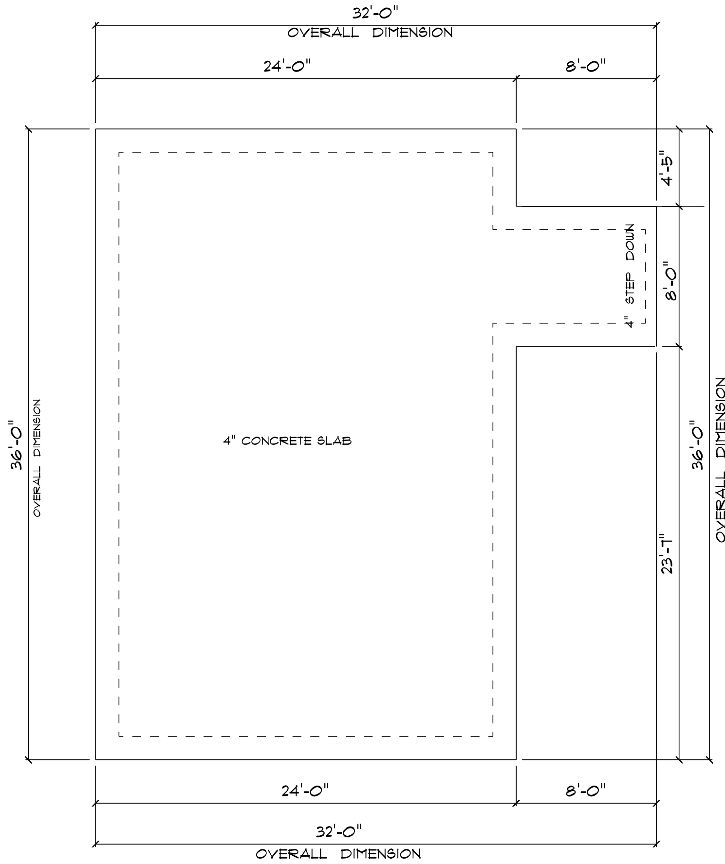
* CARPORT FOUNDATION PLAN *
