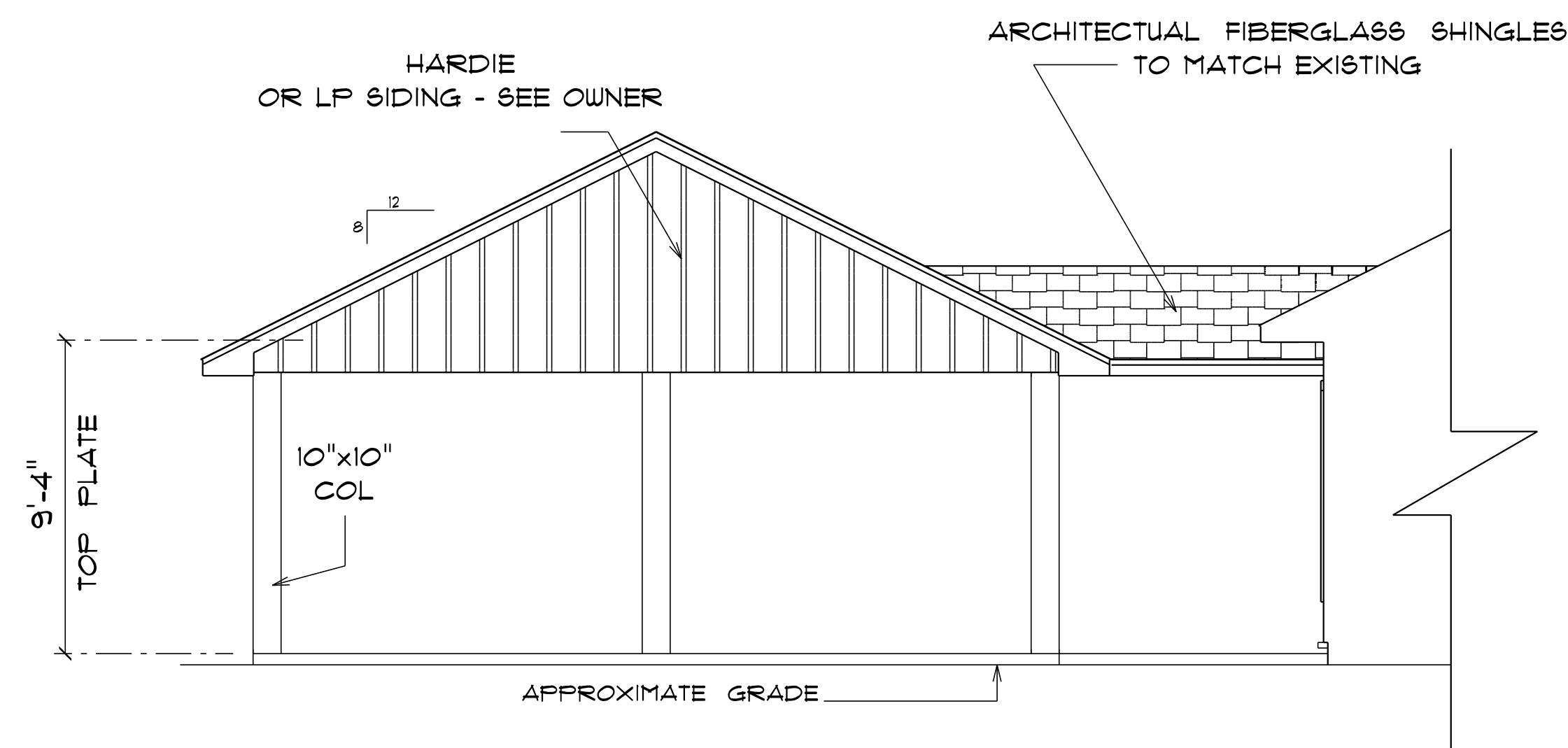
* CARPORT * * FRONT ELEVATION * SCALE : 1/4" = 1'-0"
