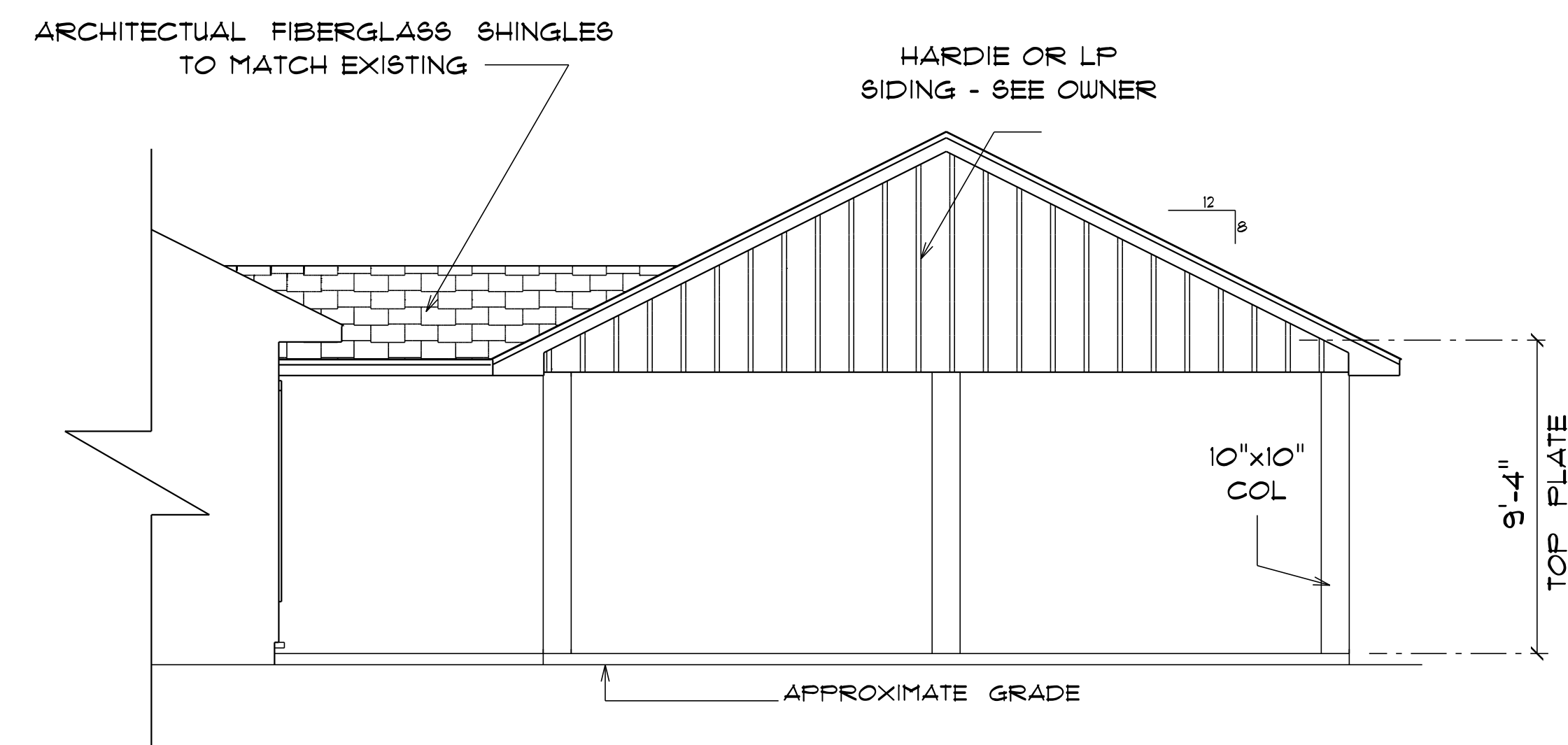
* CARPORT * * REAR ELEVATION * SCALE : 1/4" = 1'-0"
