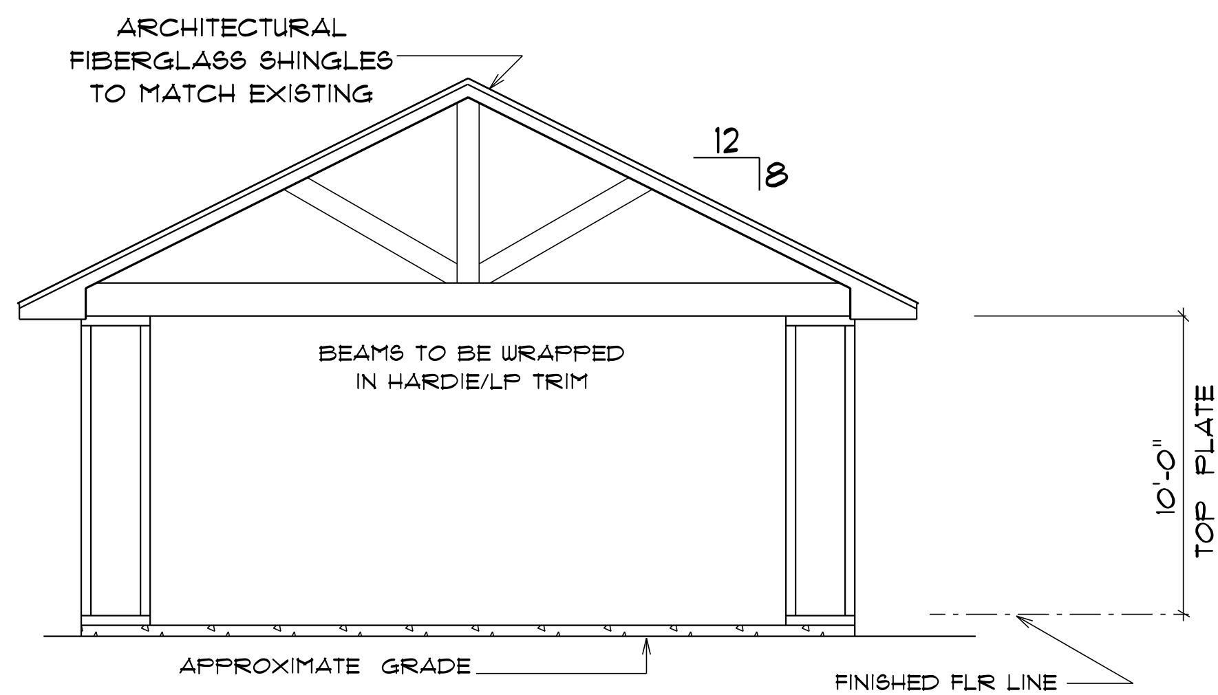
* COVERED REAR * * LEFT ELEVATION * SCALE : 1/4" = 1'-0"
