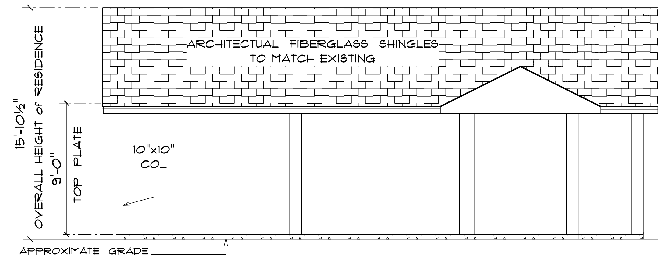
* CARPORT * * RIGHT SIDE ELEVATION * SCALE : 1/4" = 1'-0"
