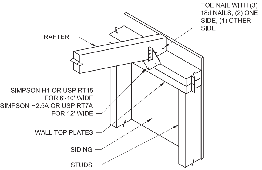
4 TRUSS TO WALL CONNECTION DETAIL SCALE: N.T.S.
