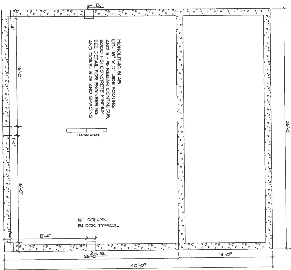
FOUNDATION / MONOLITHIC SLAB
