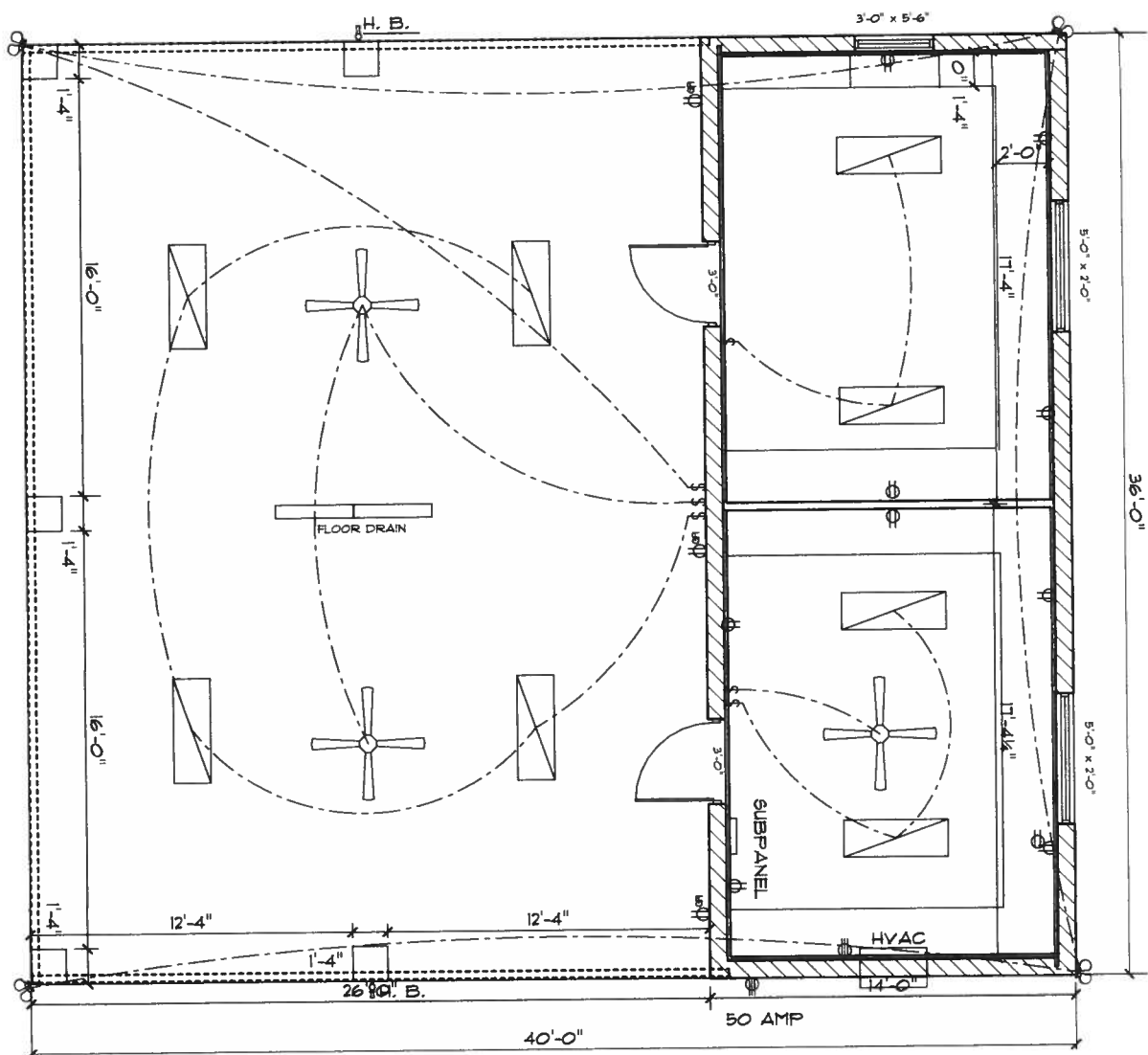
FLOOR PLAN / ELECTRICAL
