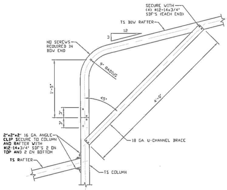
SCALE: 1/8" = 1'-0" MAXIMUM WIDTH OF SINGLE MEMBER RAFTER LEAN-TO IS 16'-0"
