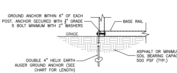
CONCRETE FOUNDATION/BASE RAIL ANCHOR DETAIL (OPEN ONLY)
