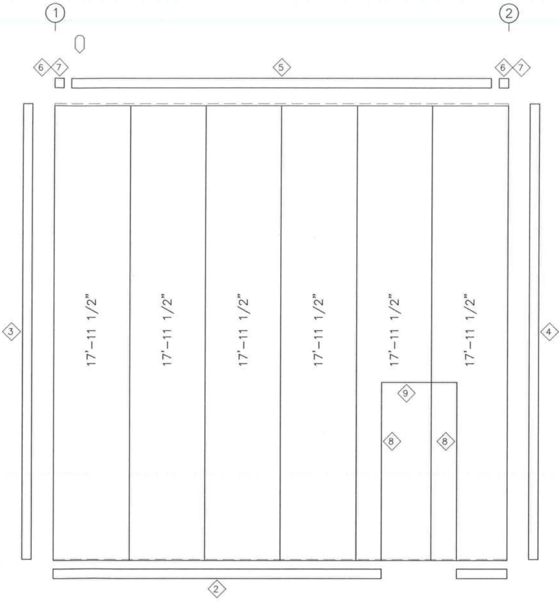
SIDEWALL SHEETING & TRIM: FRAME LINE I PANELS: 26 Ga. SX - Need Sill Poly Color
