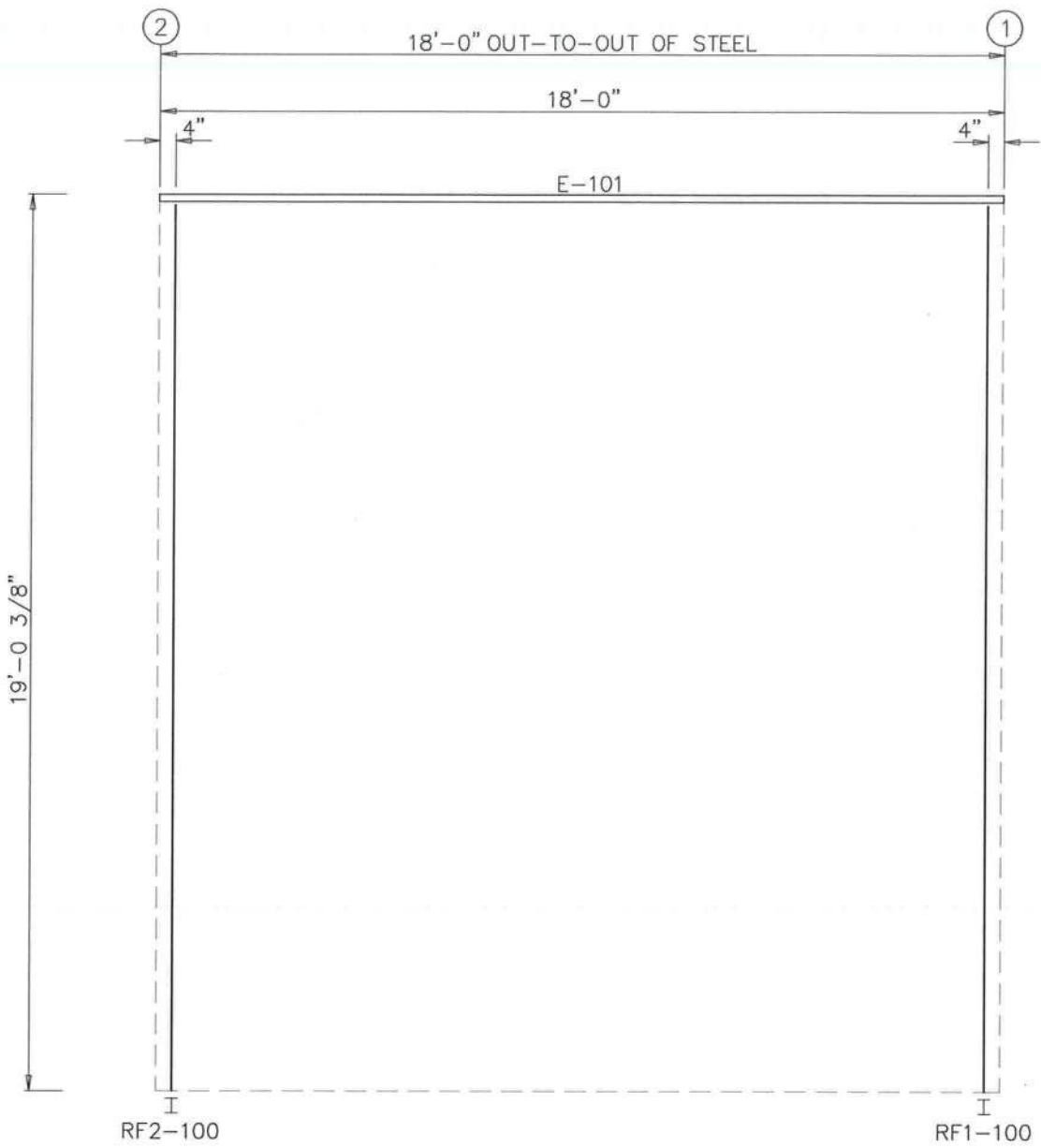
SIDEWALL FRAMING: FRAME LINE B
