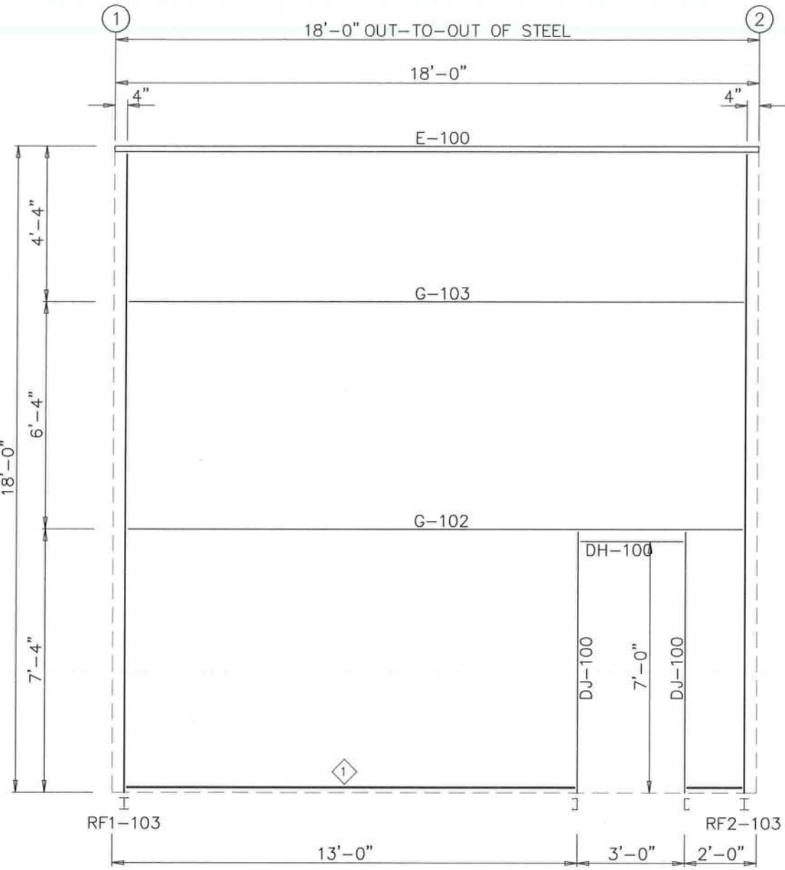
SIDEWALL FRAMING: FRAME LINE I
