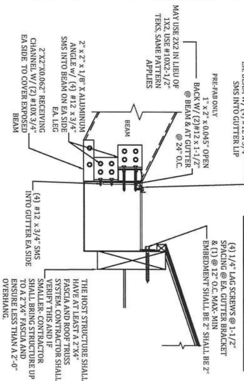
A GUTTER BRACKET & BEAM ATTACHMENT DETAIL N.T.S.
