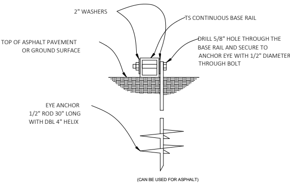
3B GROUND BASE HELIX ANCHORAGE SCALE: NTS
