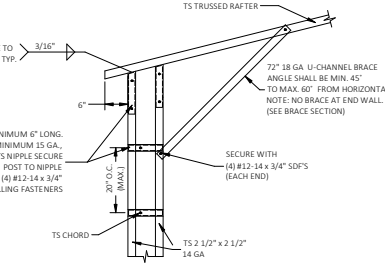
1B BOX EAVE RAFTER COLUMN CONNECTION DETAIL FOR HEIGHTS 16'-0" < TO <= 20'-0" SCALE: NTS
