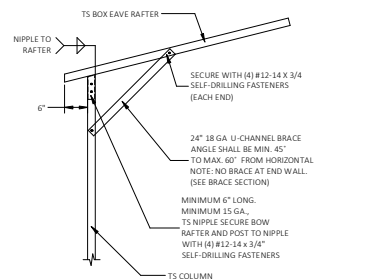
1.2 BOX EAVE RAFTER COLUMN CONNECTION DETAIL FOR HEIGHTS 12'-0" < TO <= 13'-0" SCALE: NTS
