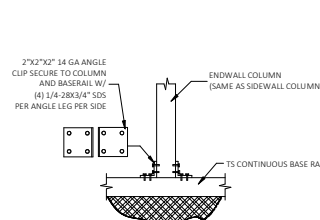
2C ENDWALL COLUMN/BASE RAIL CONNECTION DETAIL SCALE: NTS
