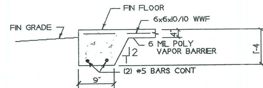
TYPICAL TURNDOWN NOT TO SCALE
