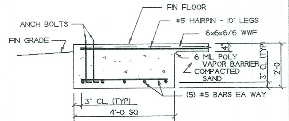
TYPICAL FOOTING SECTION NOT TO SCALE
