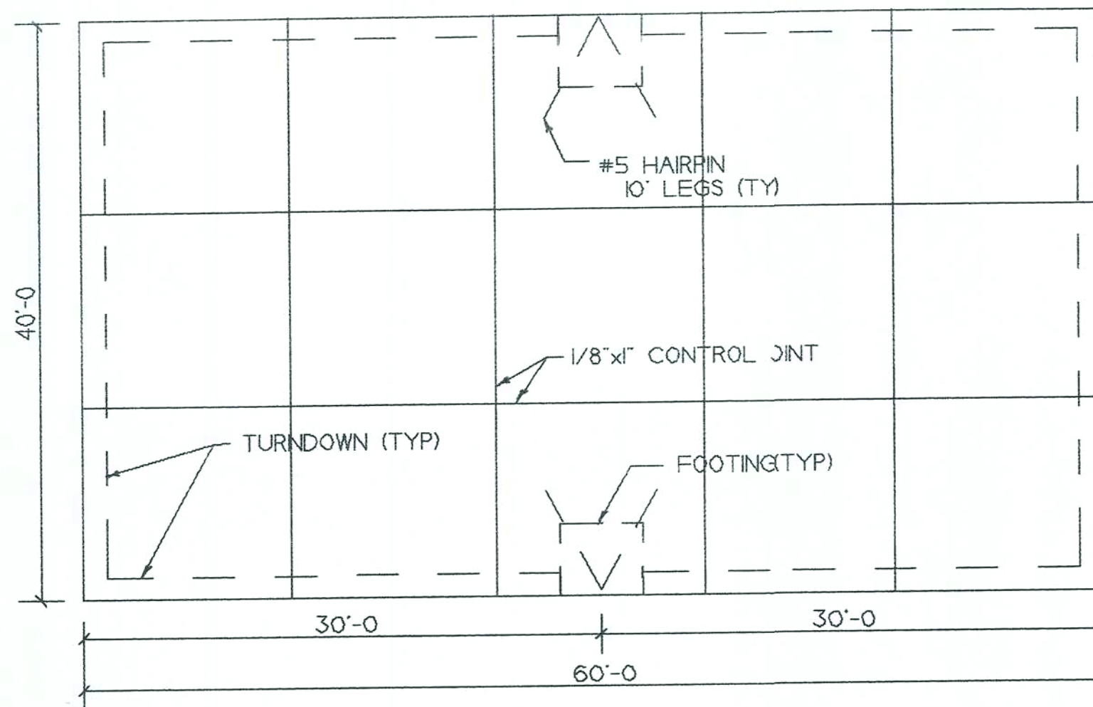
FOUNDATION PLAN NOT TO SCALE
