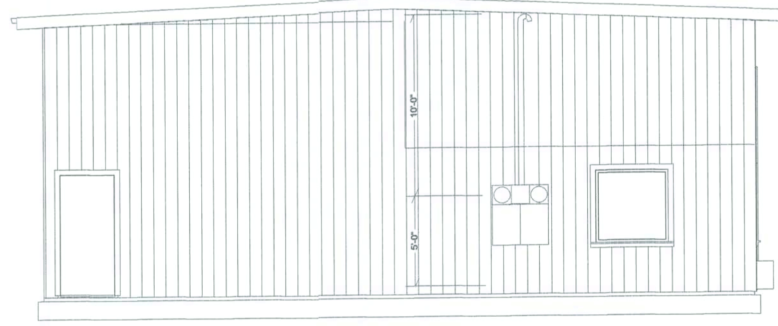
LEFT ELEVATION
