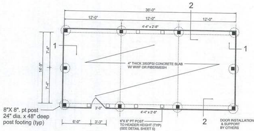
FOUNDATION PLAN VIEW
