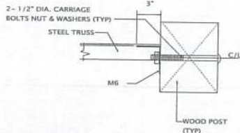
TRUSS TO POST DETAIL PLAN VIEW
