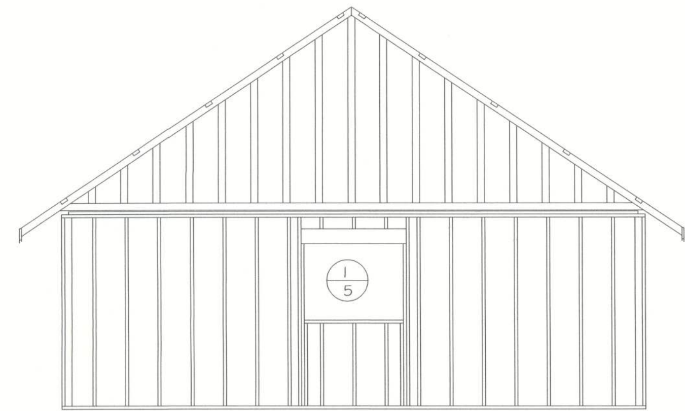
RIGHT SIDE WALL FRAMING ELEVATION
