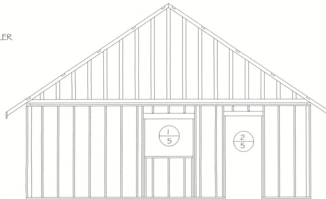
LEFT SIDE WALL FRAMING ELEVATION
