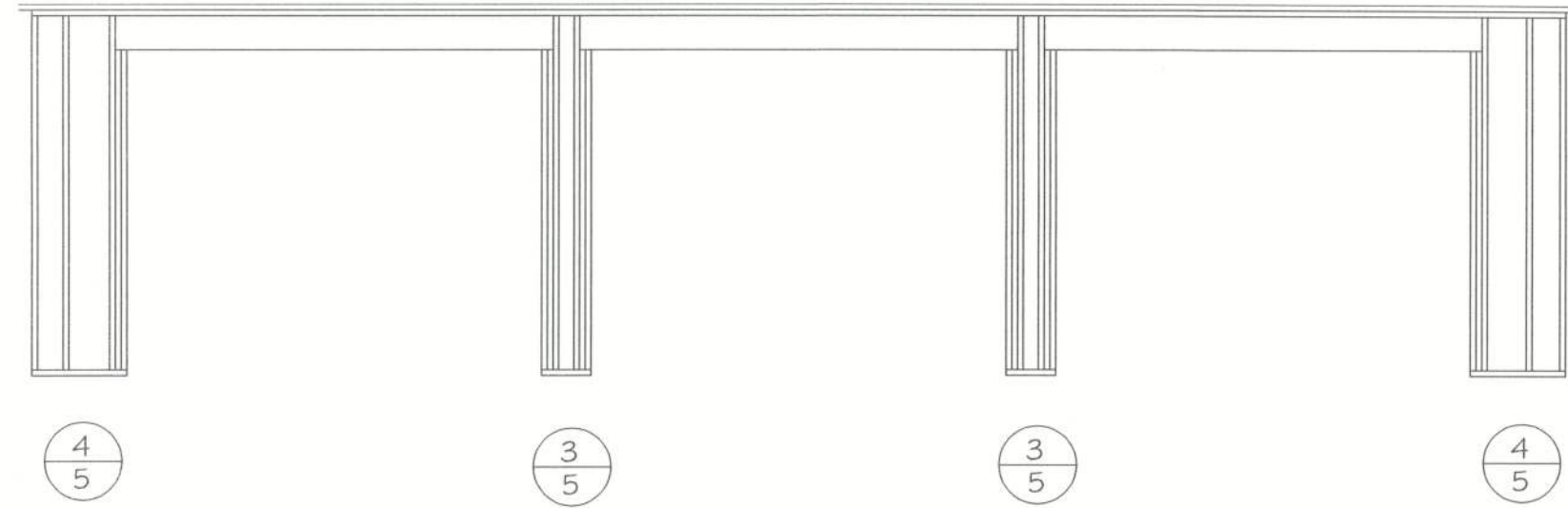
FRONT WALL FRAMING ELEVATION
