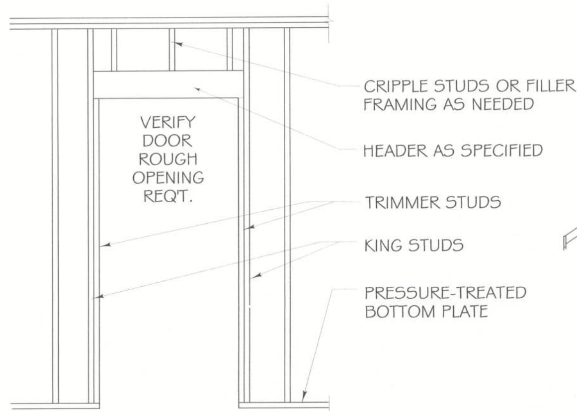
2 DOOR OPENING DETAIL
