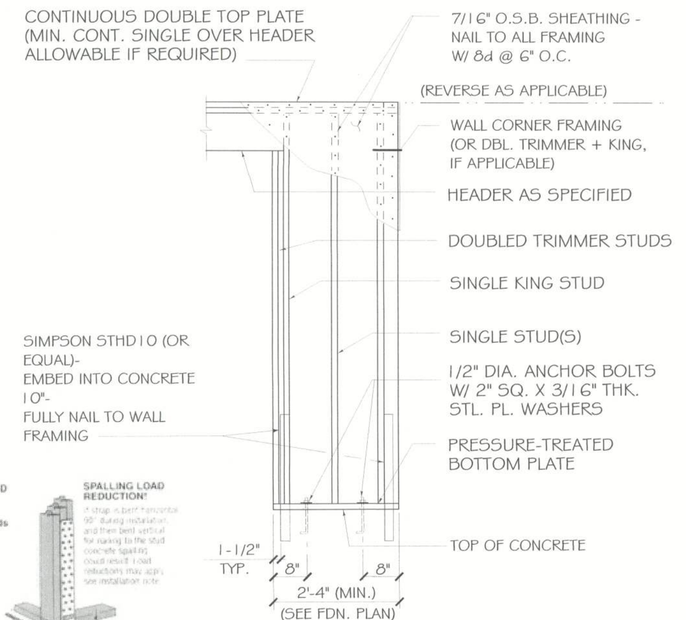
4 ALTERNATE BRACED WALL PANEL DETAIL
