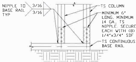
COLUMN/BASE RAIL CONNECTION DETAIL
