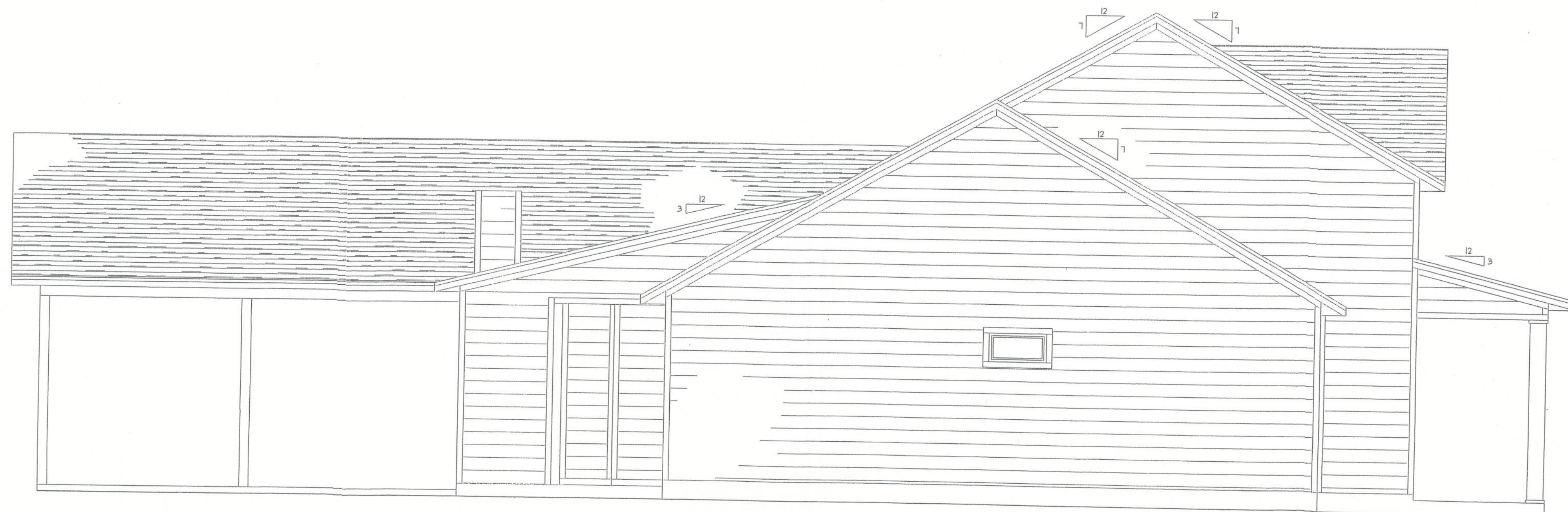
LEFT ELEVATION
