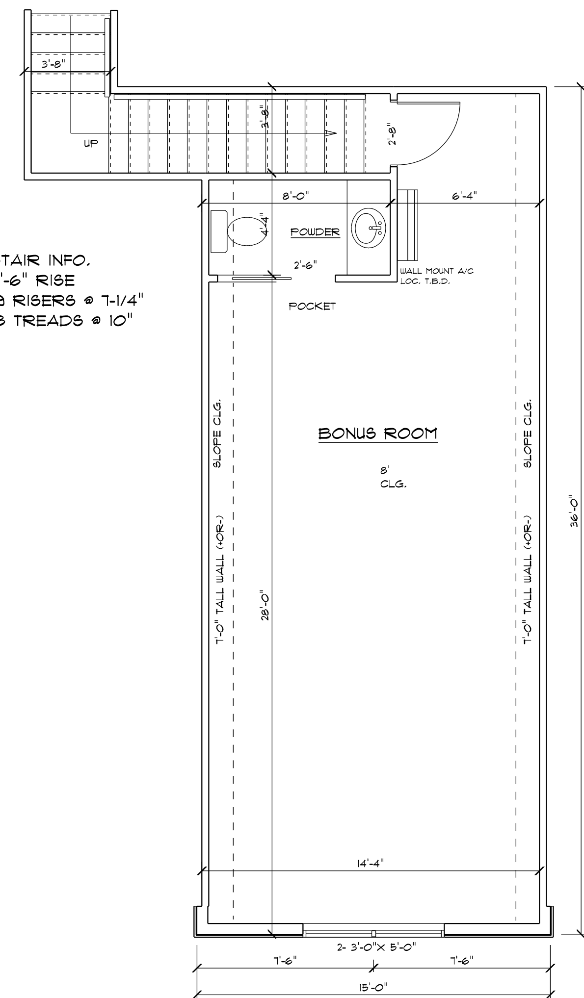
BONUS ROOM FLOOR PLAN
