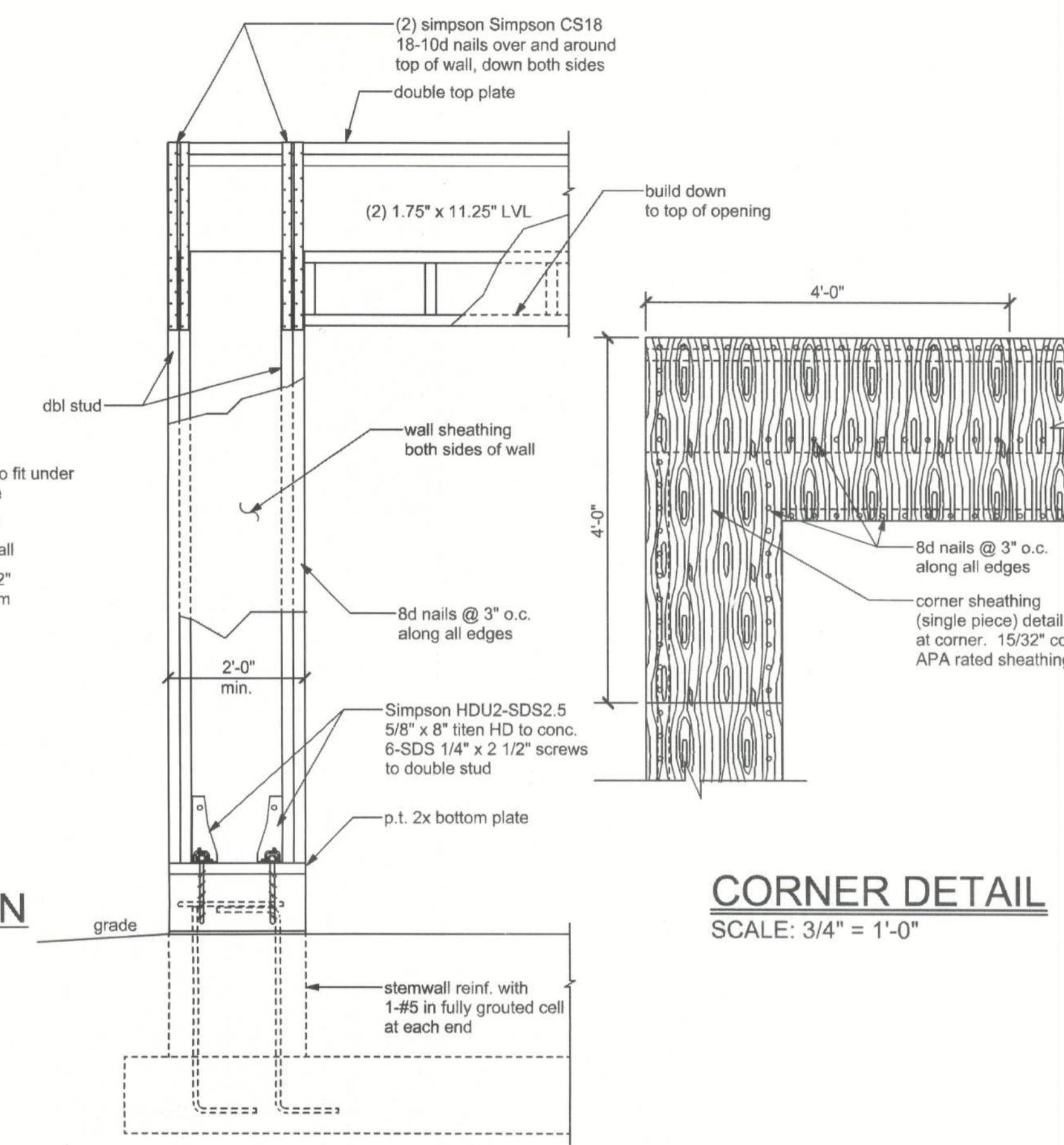
GARAGE ENDWALL SHEATHING DETAILS SCALE: 3/4" = 1'-0"
