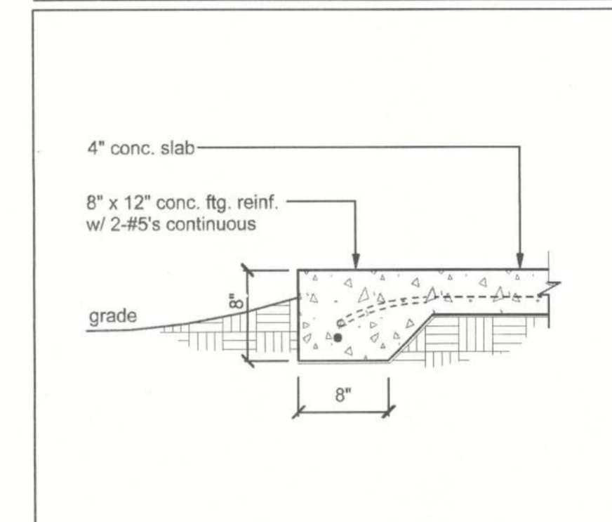
4 THICKENED EDGE AT STOOP SCALE: 1" = 1'-0"
