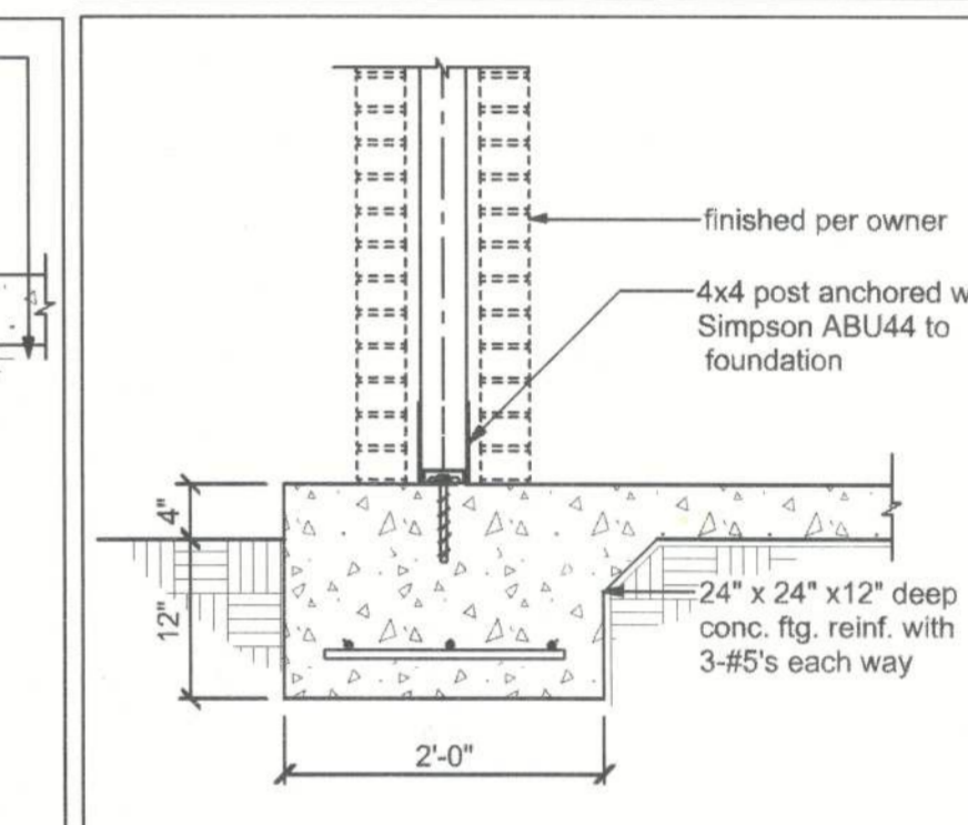
6 COLUMN/FOOTING DETAIL SCALE: 3/4" = 1'-0"
