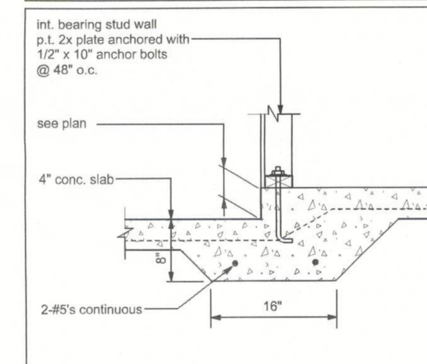
7 FOOTING STEP AT INTERIOR MONO
