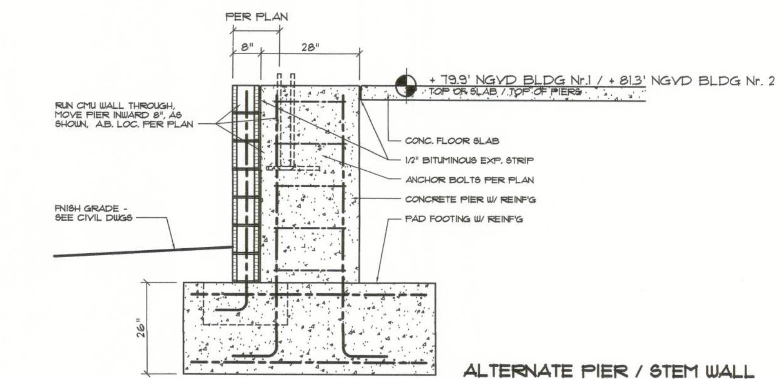
STEM WALL / PIER SECTIONS SCALE: NONE III
