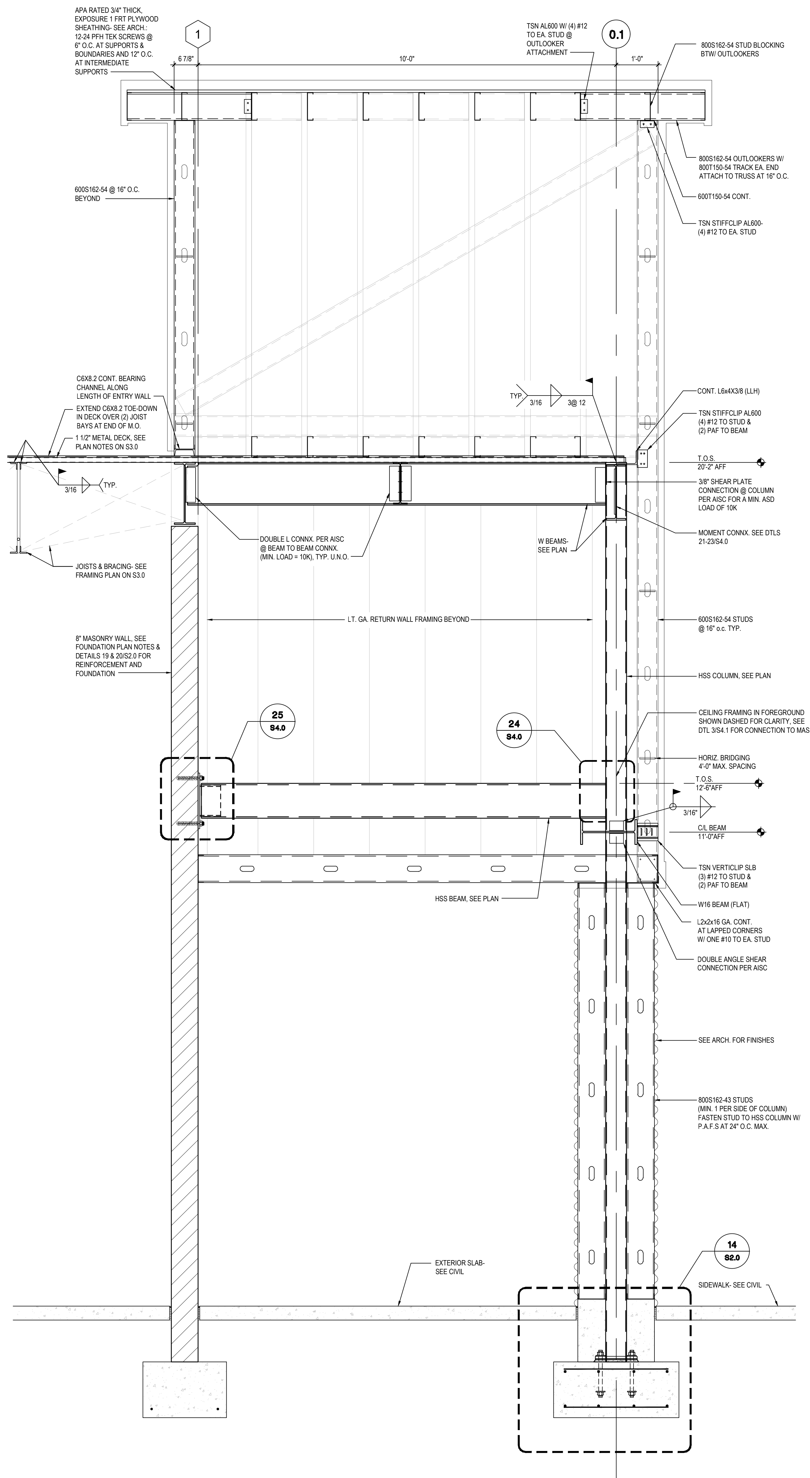
B | SECTION 3/4" = 1'-0"
