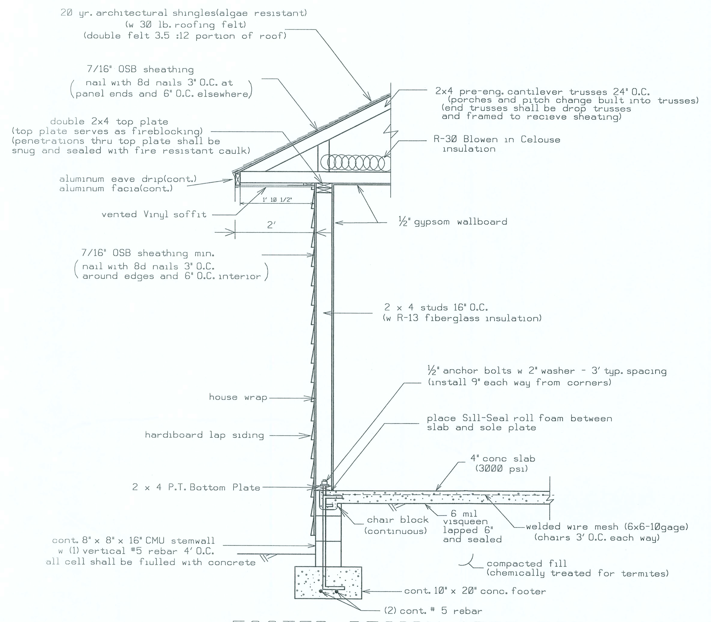
FOOTER DESIGN 1000 PSF
