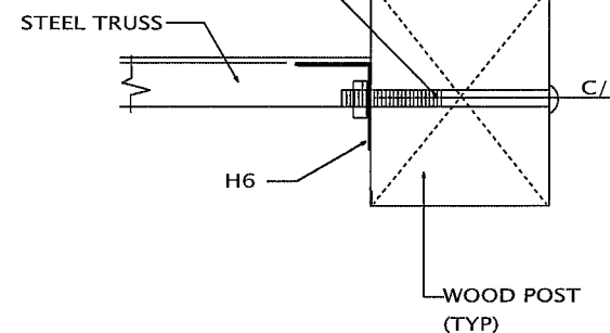
TRUSS TO POST DETAIL PLAN VIEW
