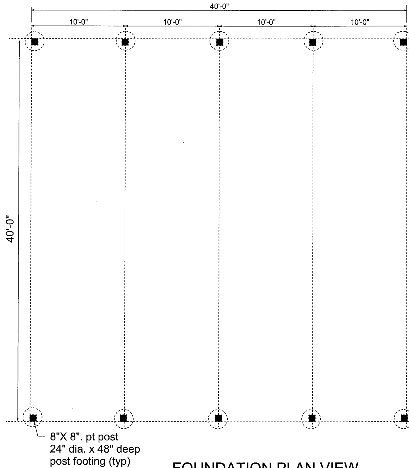
FOUNDATION PLAN VIEW
