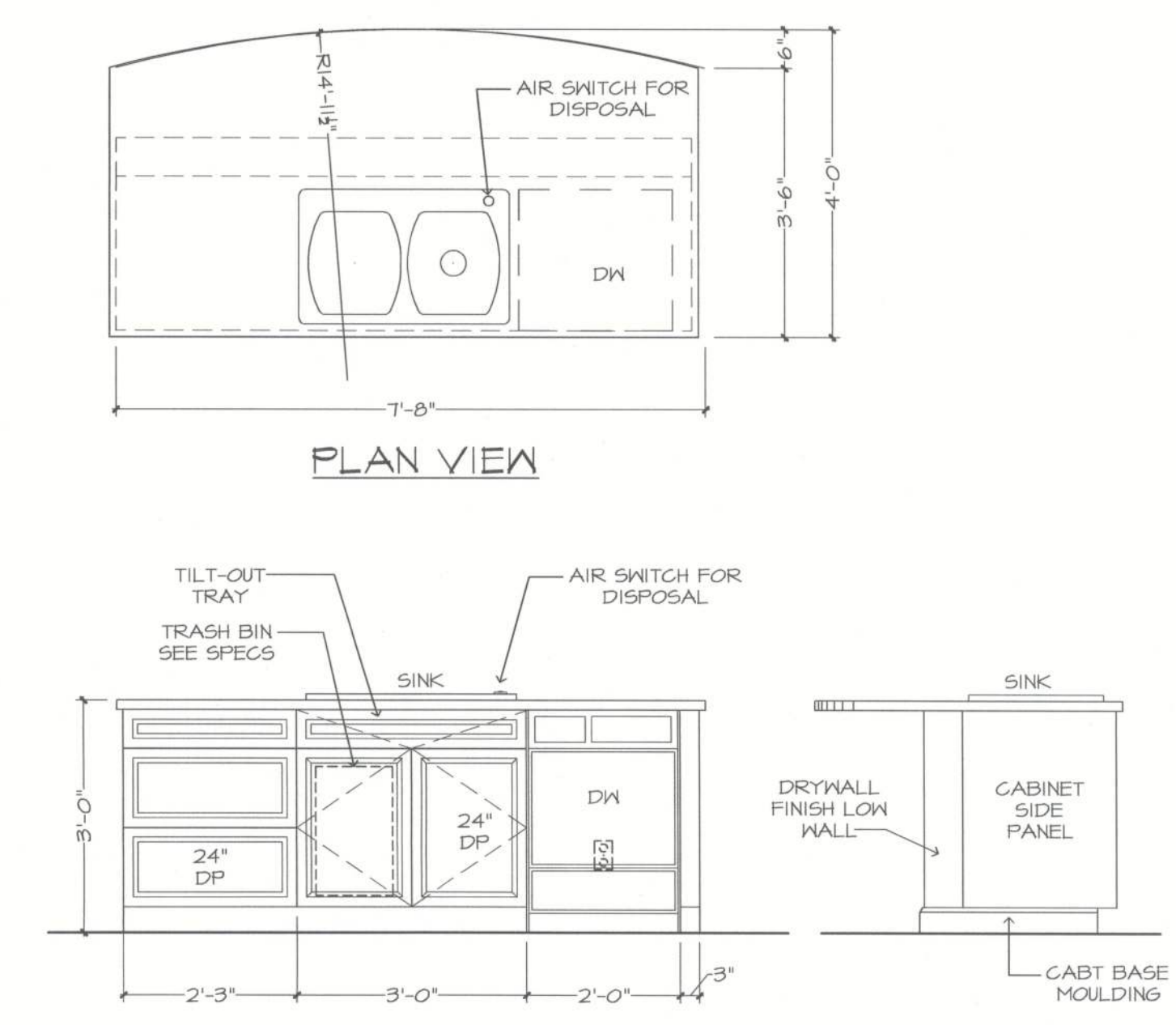
FRONT VIEW KITCHEN ISLAND TYP. SIDE VIEW
