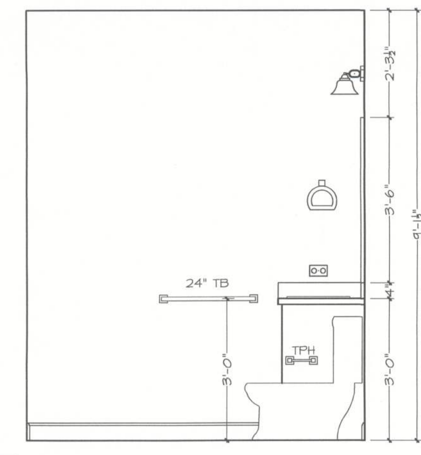
WALL "Z"
