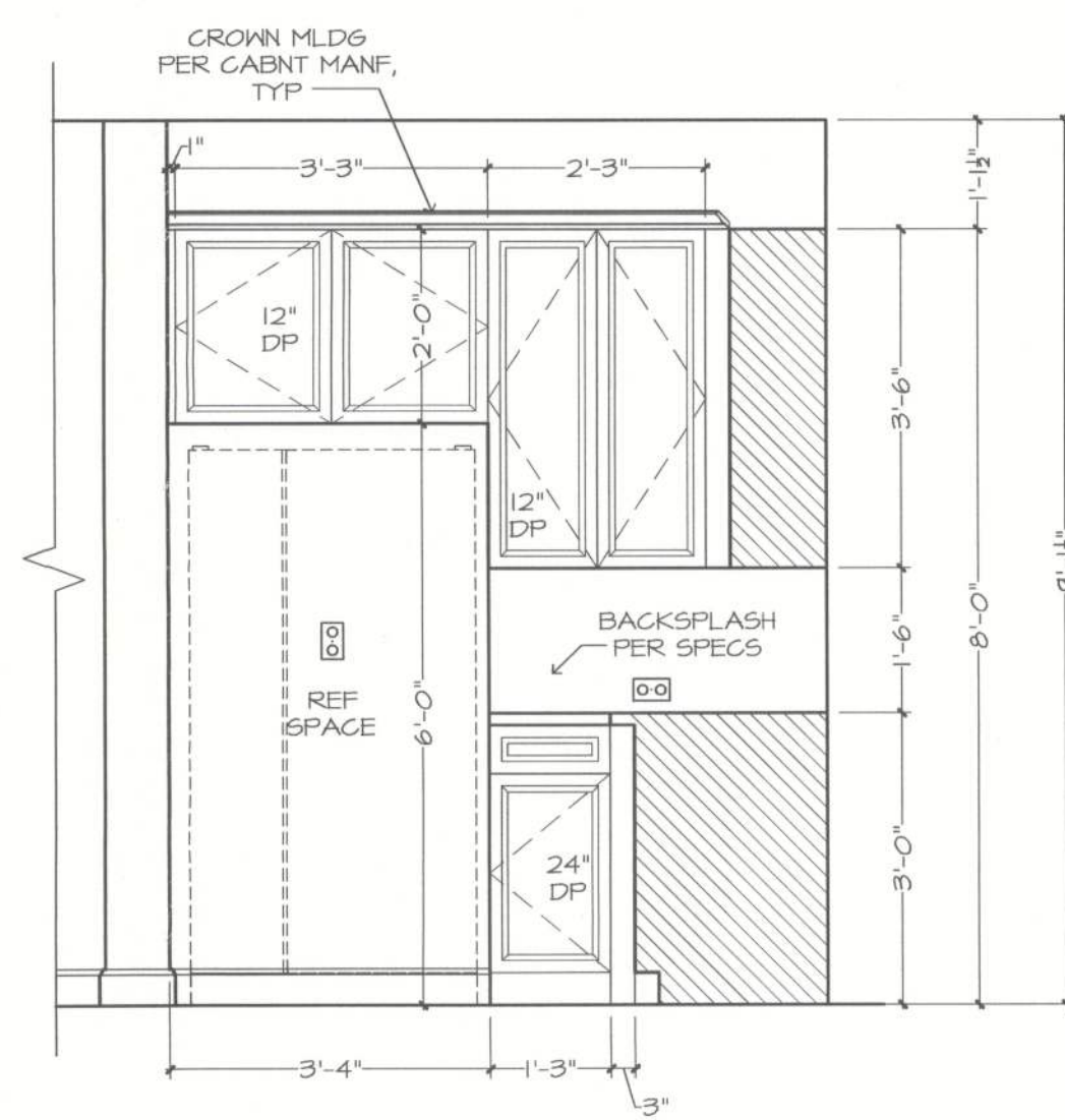
WALL "Z"
