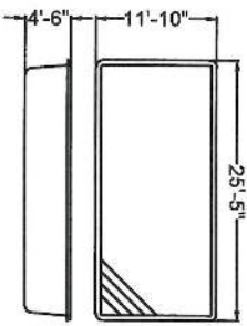
DELRAY - B 8,100 gal. approx.
