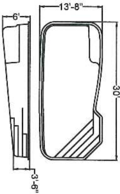
CARMEL - FF 12,000 gal. approx.
