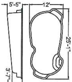
FREEPORT - FP 6,000 gal. approx.
