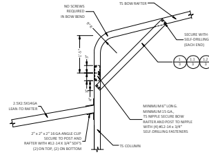
TYPICAL BOW RAFTER LEAN-TO OPTIONS FRAMING SECTION
