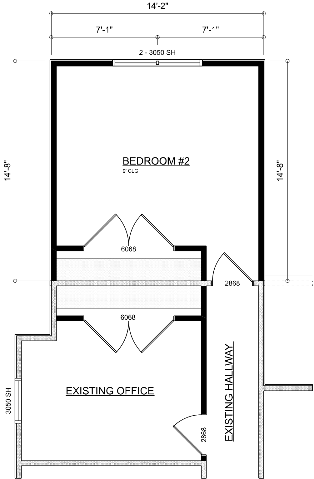
DIMENSIONED FLOOR PLAN SCALE: 1/4" = 1'-0"
