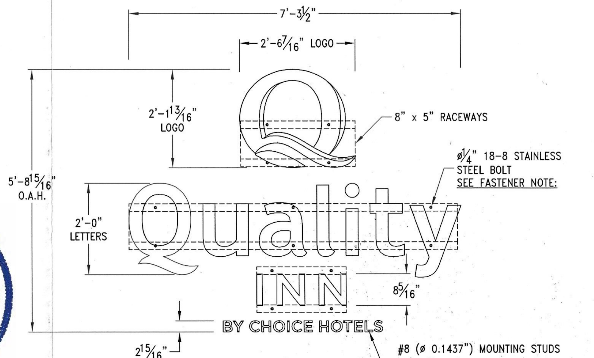
ELEVATION VIEW
