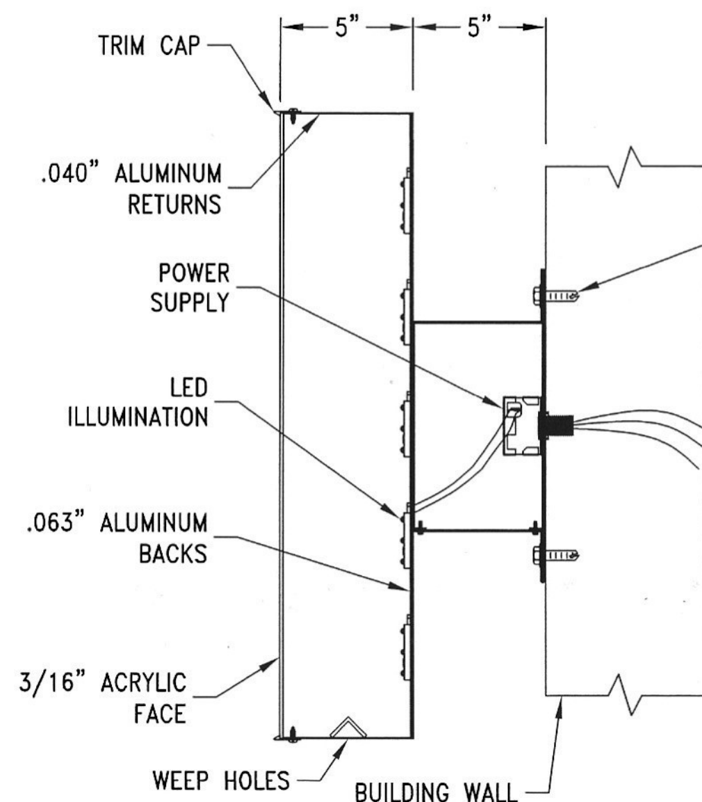
CHANNEL LOGO / LETTER DETAIL VIEW
