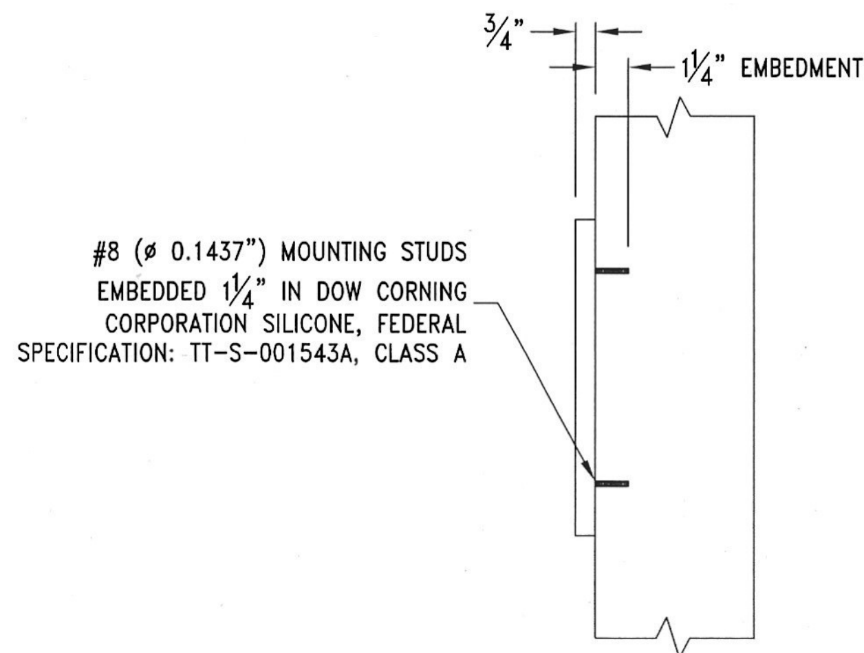
FLAT CUT PVC LETTER DETAIL VIEW
