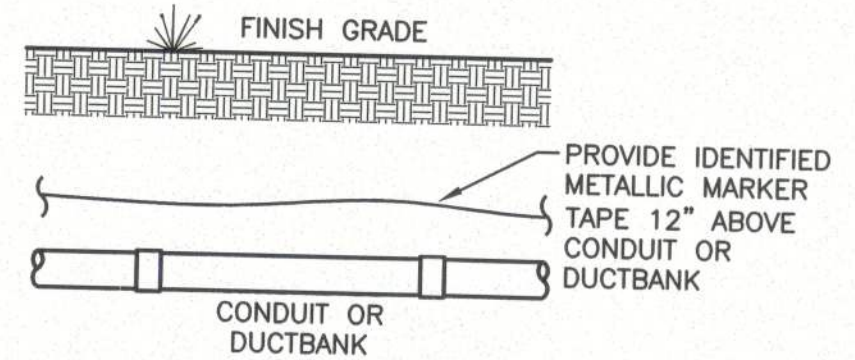
BURIED CONDUIT MARKER DETAIL
