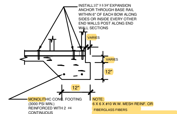
1 CONCRETE BASE RAIL ANCHORAGE SCALE: NTS (OPTIONAL)
