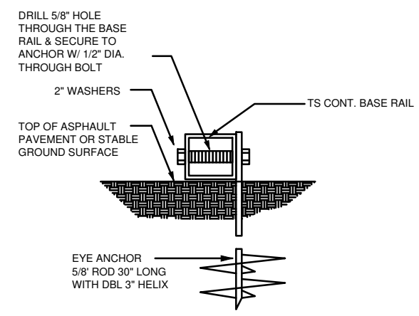
4 BASE RAIL ANCHORAGE SCALE: NTS
