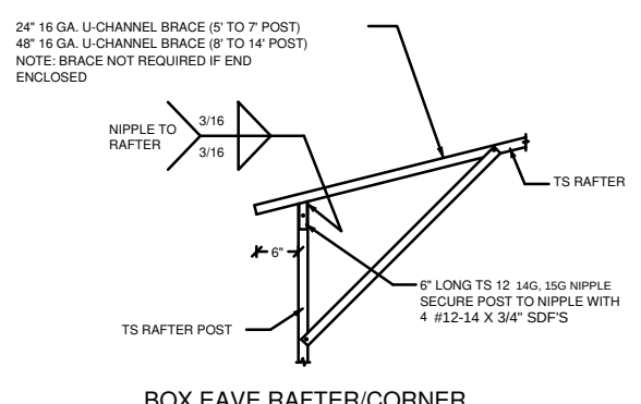
3 BOX EAVE RAFTER/CORNER POST DETAIL SCALE: NTS
