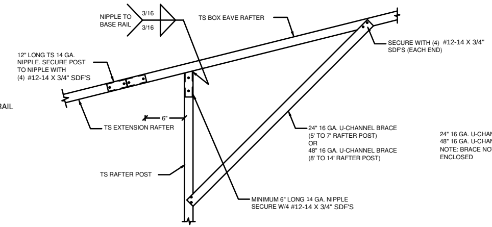
5 SIDE EXTENSION RAFTER/CORNER POST DETAIL SCALE: NTS
