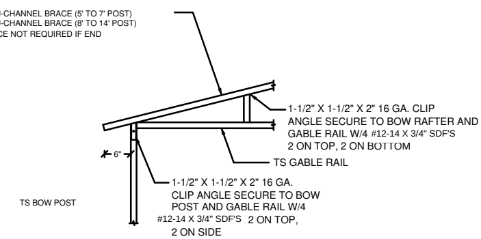
6 GABLE RAIL TO RAFTER POST CONNECTION DETAIL SCALE: NTS
