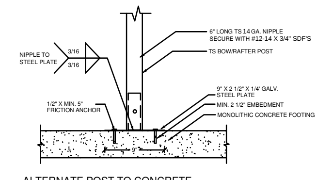
ALTERNATE POST TO CONCRETE FOUNDATION CONNECTION DETAIL SCALE: NTS
