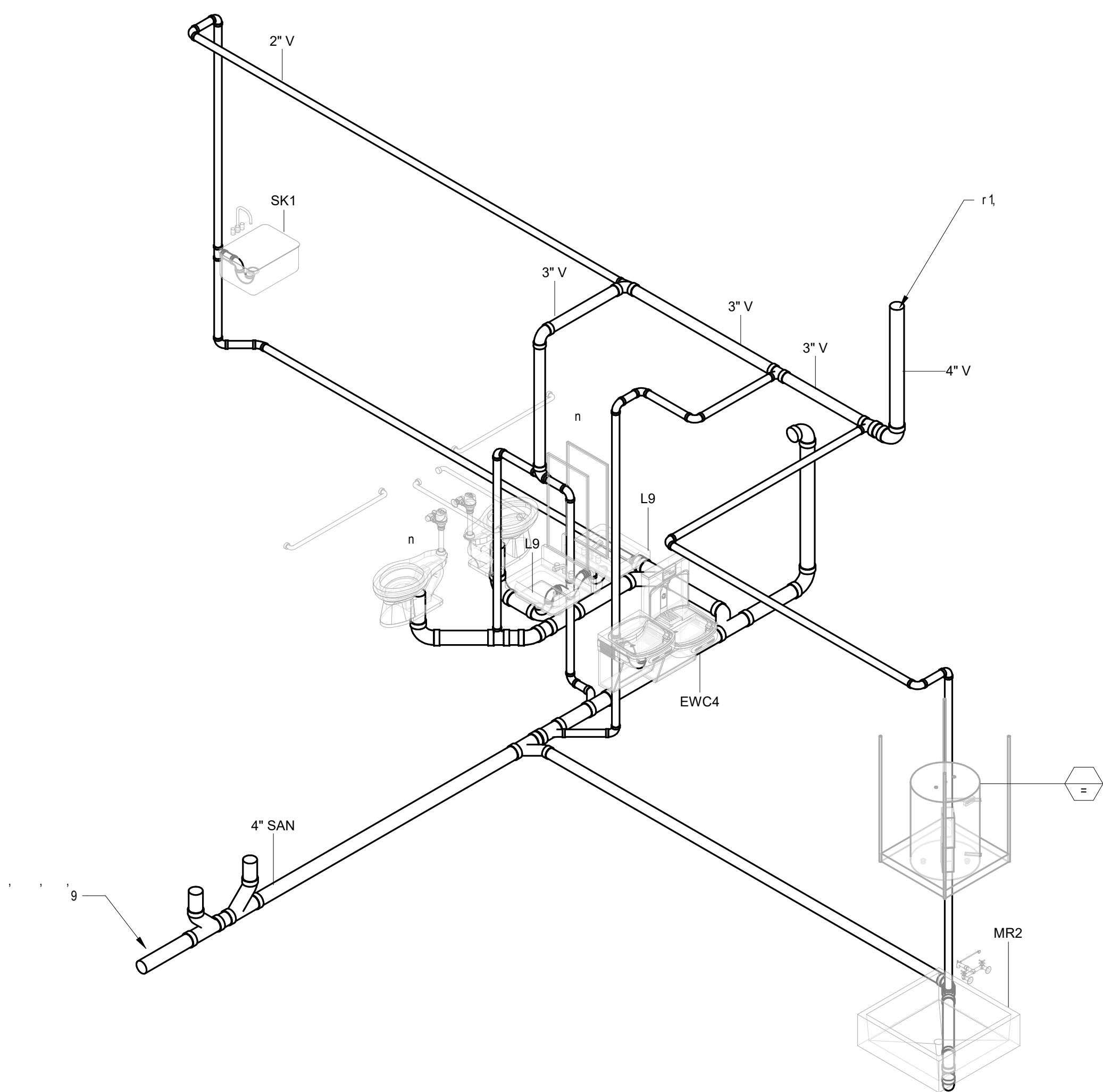
PLUMBING - SANITARY WASTE AND VENT RISER DIAGRAM
