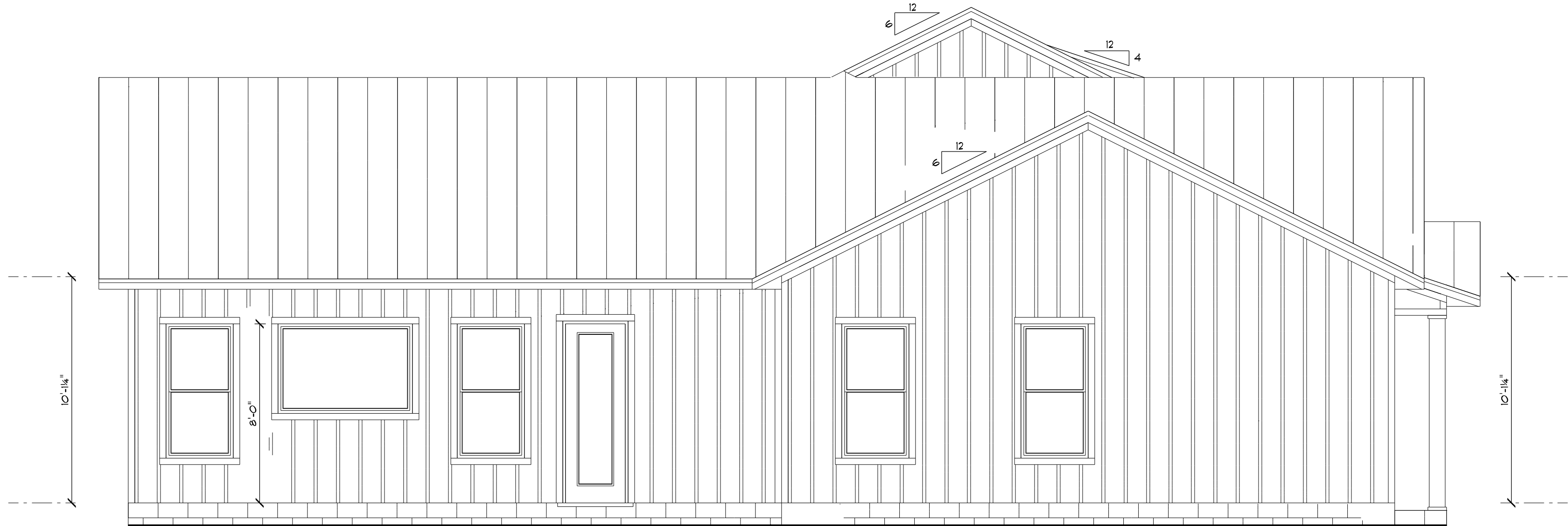
LEFT ELEVATION
