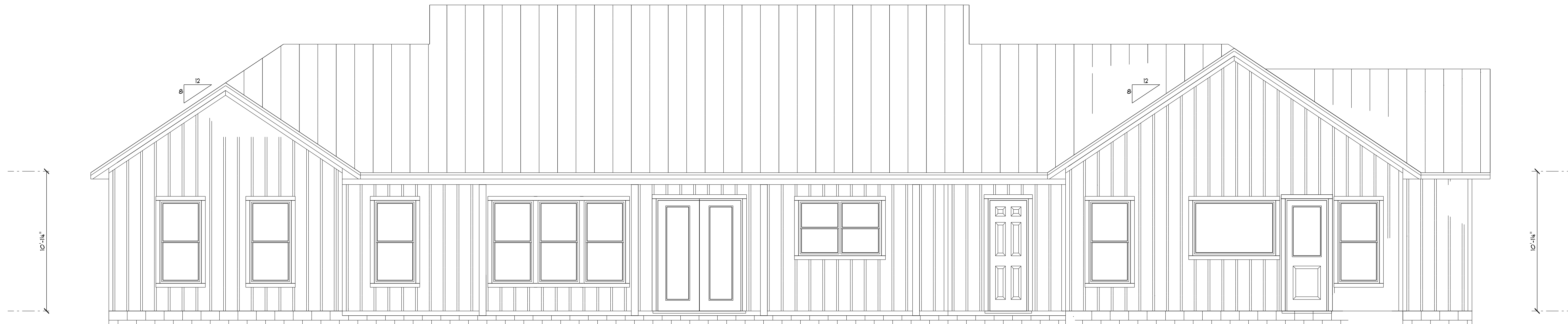
REAR ELEVATION
