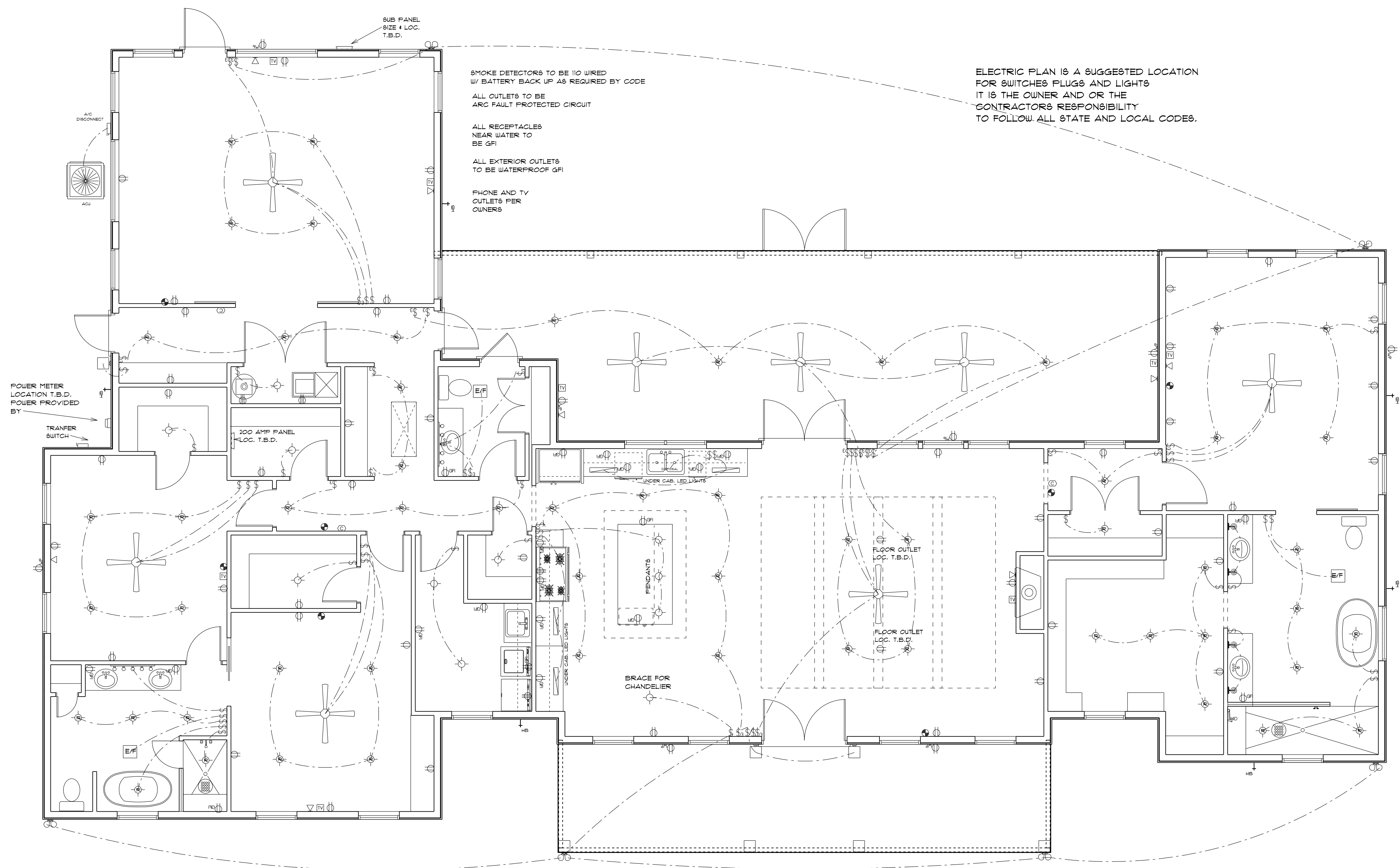
ELECTRICAL PLAN
