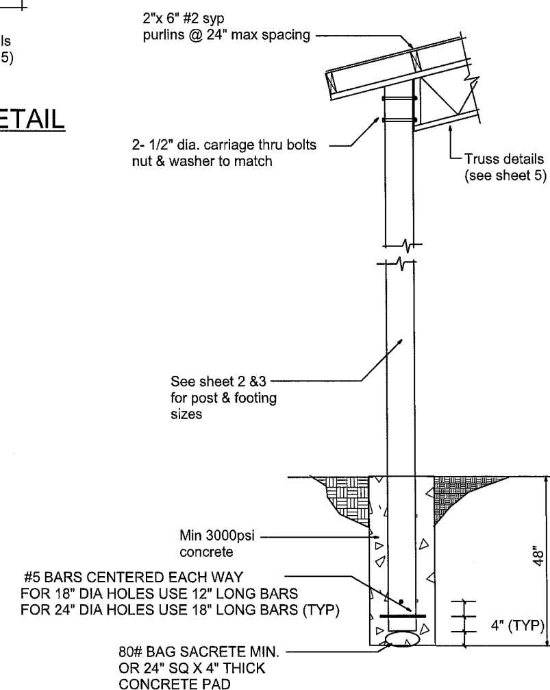
POST FOOTING TO TRUSS DETAIL
