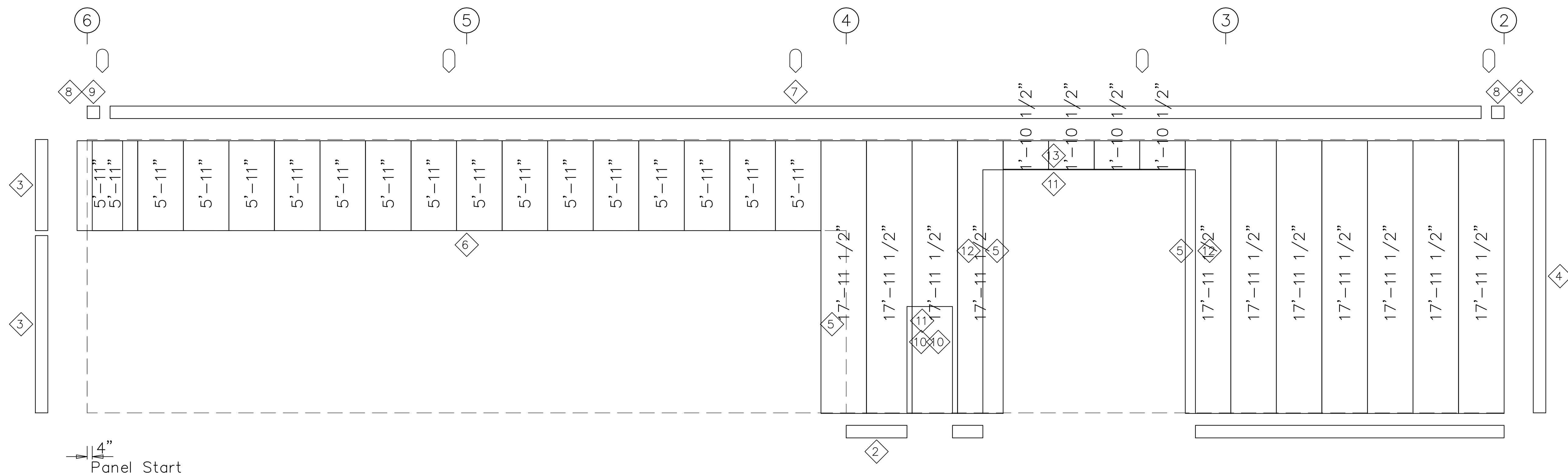
SIDEWALL SHEETING & TRIM: FRAME LINE A
