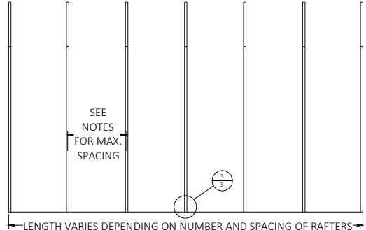
TYPICAL RAFTER/COLUMN SIDE FRAME SECTION
