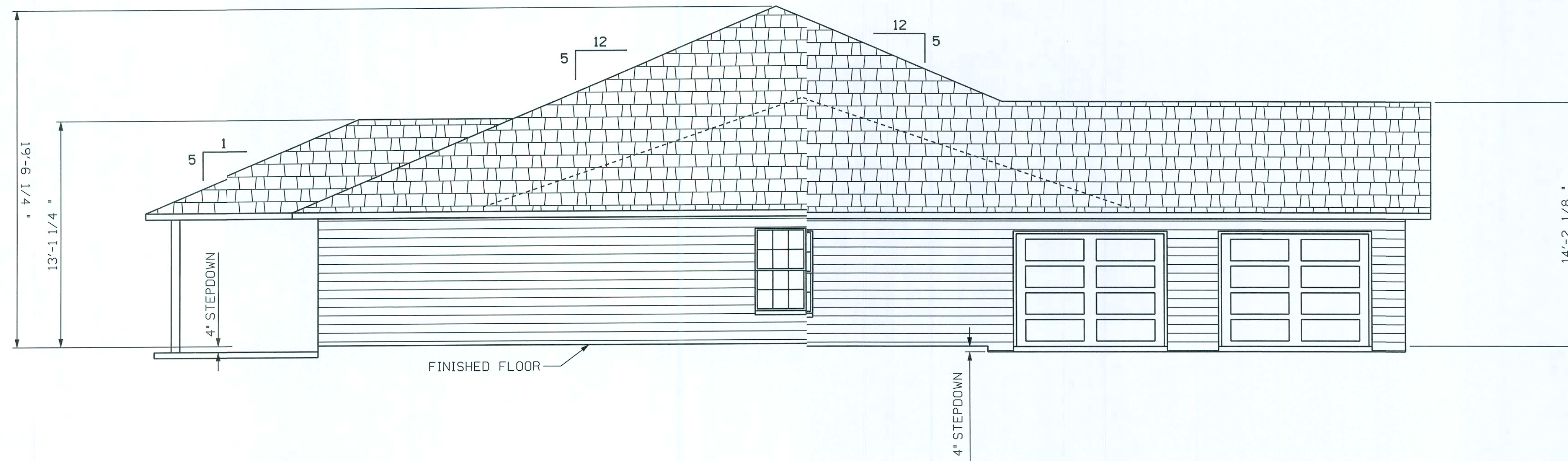
LEFT ELEVATION
