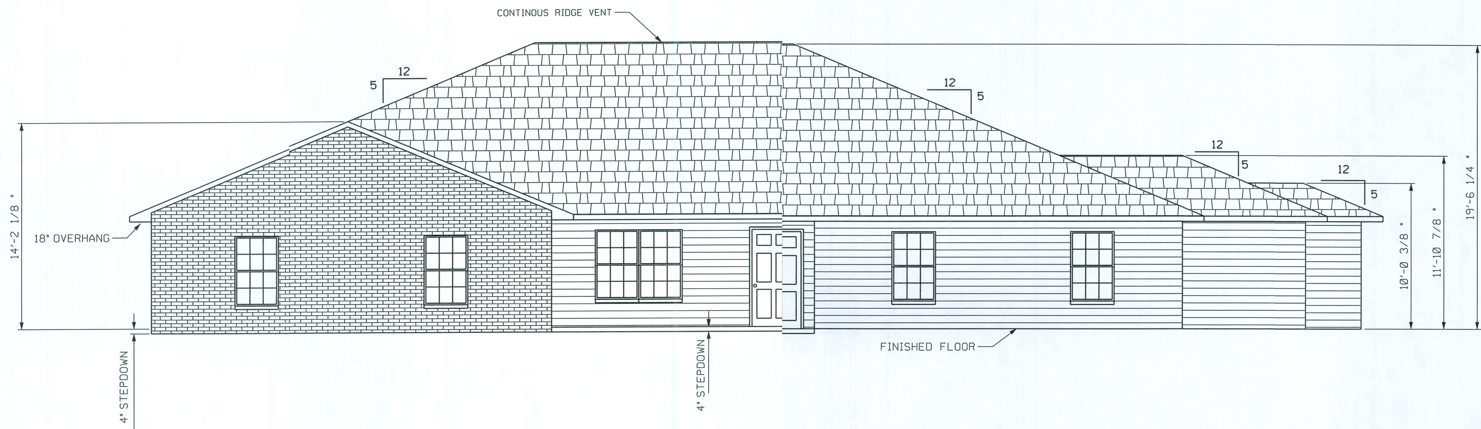
FRONT ELEVATION
