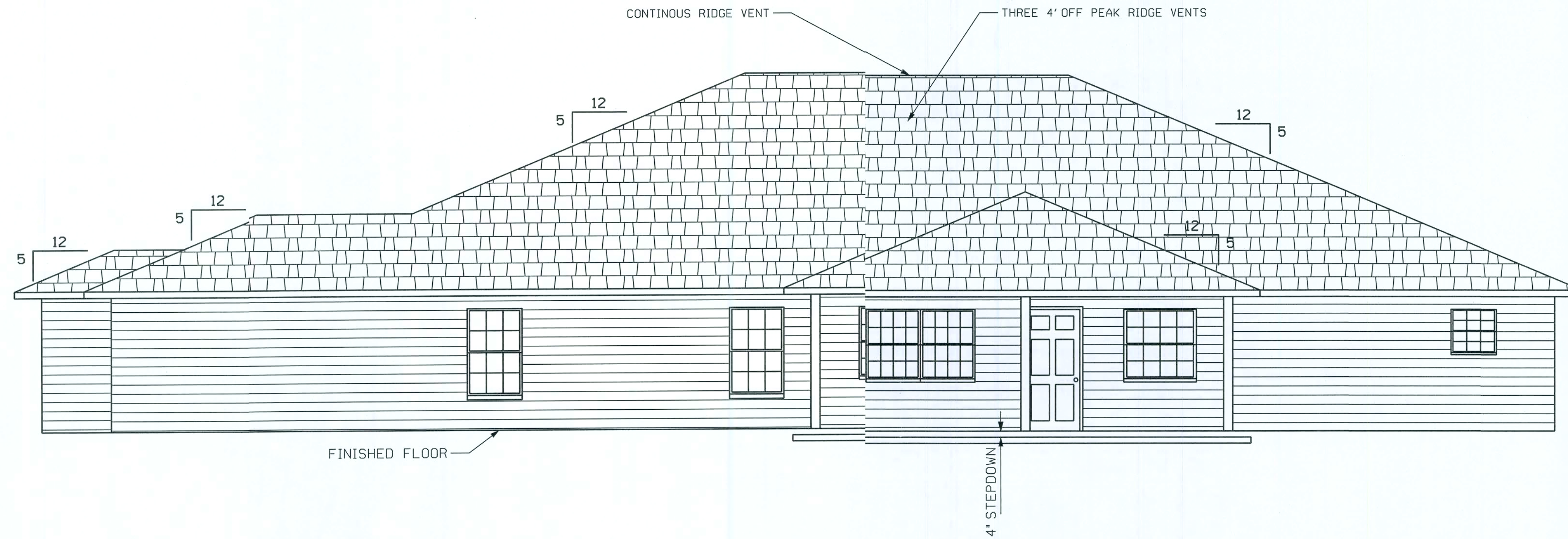
REAR ELEVATION
