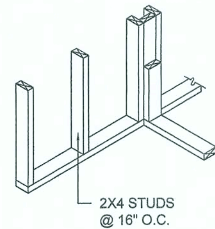
WALL INTERSECTION
