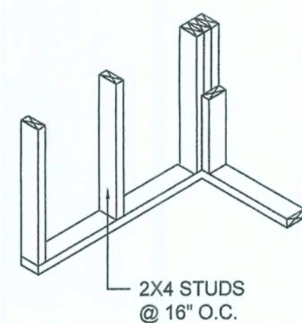
WALL CORNER
