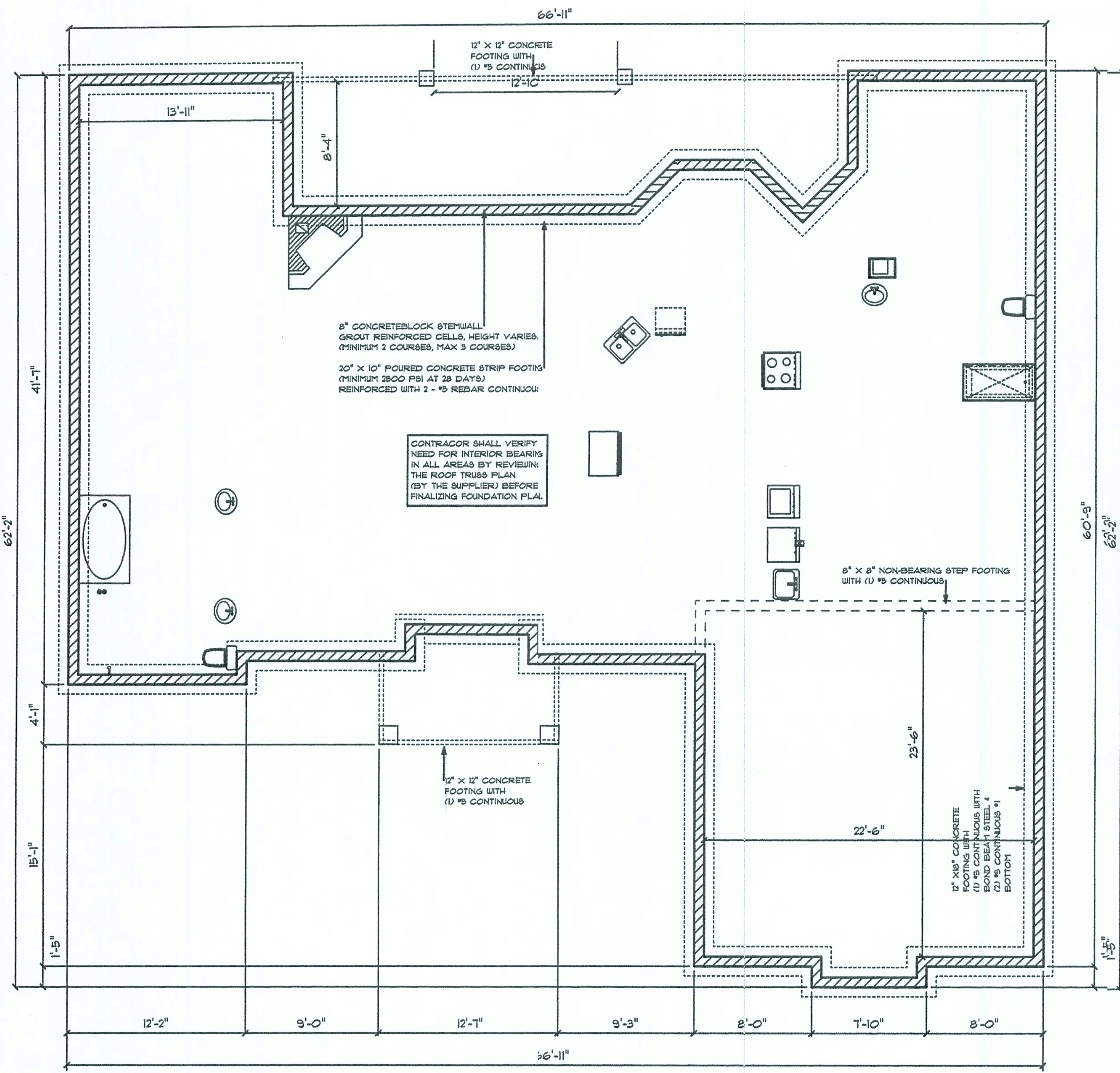
FOUNDATION PLAN
