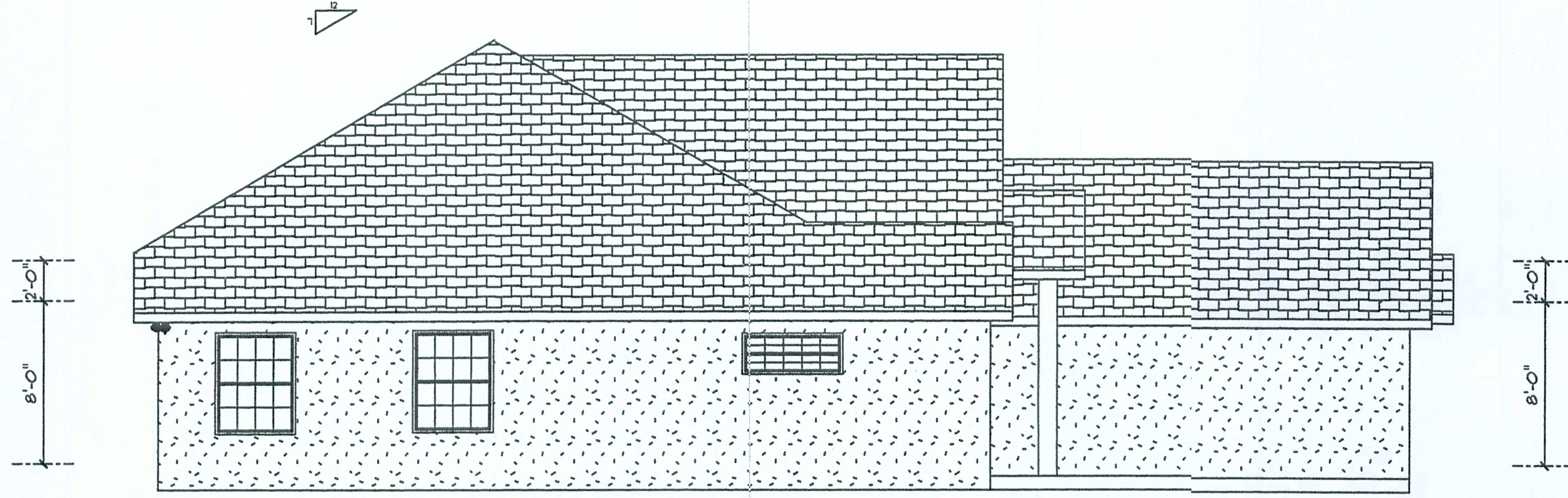
LEFT ELEVATION
