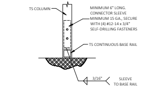
2 SIDEWALL SINGLE COLUMN/BASE RAIL CONNECTION DETAIL SCALE: NTS
