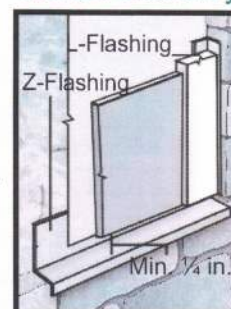
Figure 11 Mortar/Masonry
