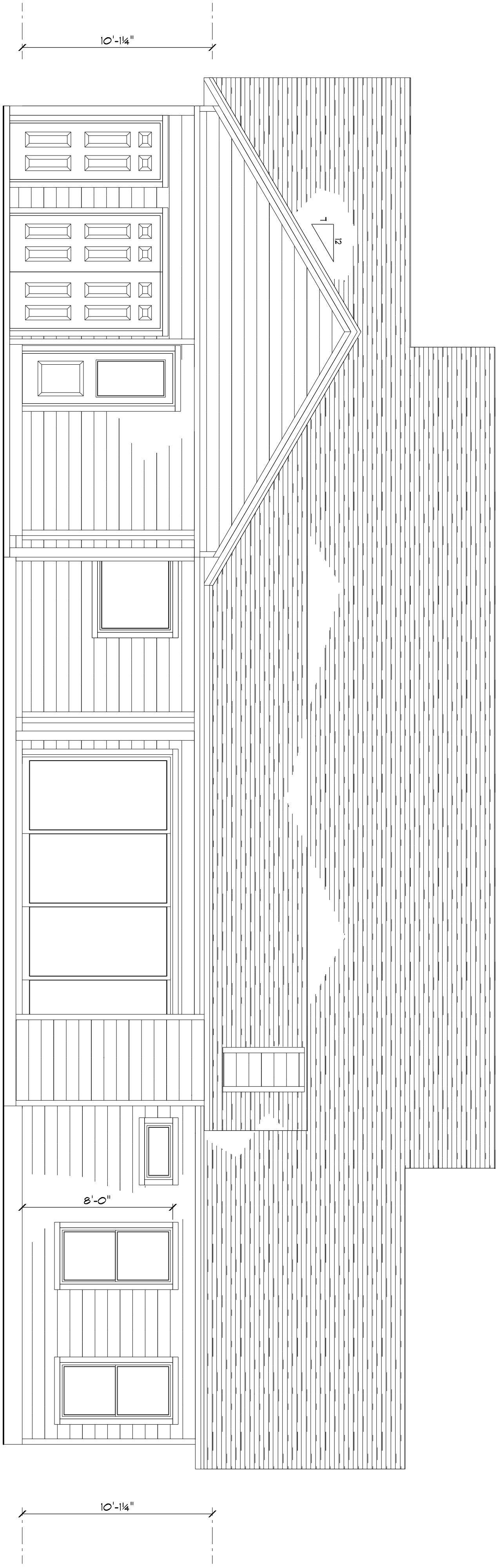
REAR ELEVATION
