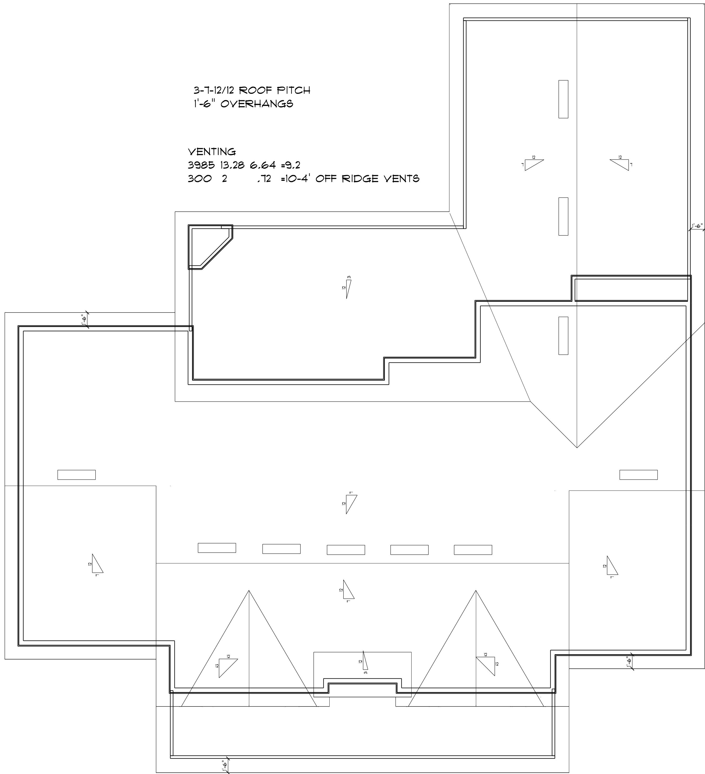
ROOF PLAN 3/16" SCALE
