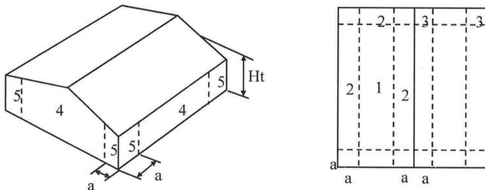
Figure 6-5 - External Pressure Coefficients, GC_p Loads on Components and Cladding for Buildings w/ H_t \leq 60 ft
