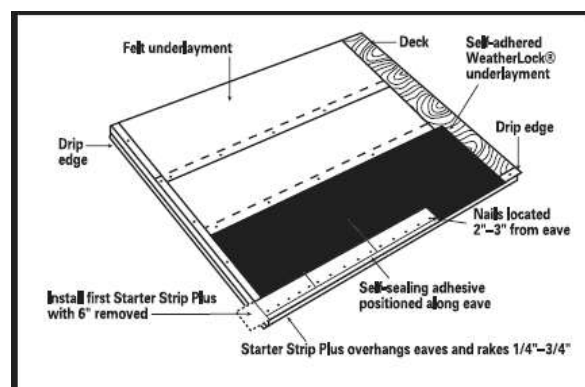
Figure 2: Minimum Nailing, Starter Strip Plus
