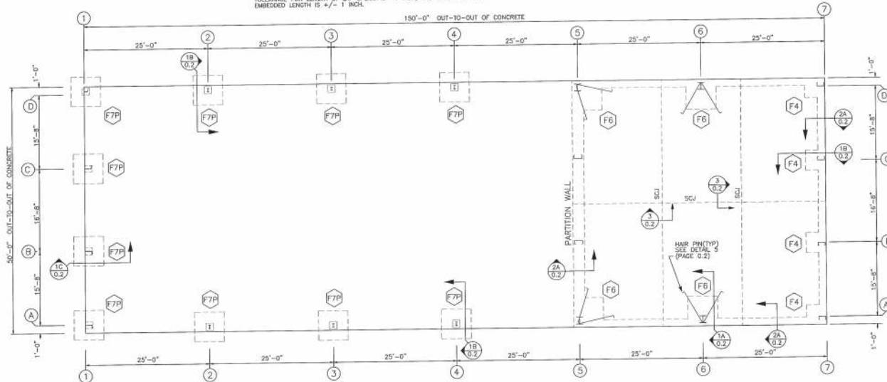
FOUNDATION PLAN LAYOUT NOTE: All Base Plates @ 100'-0" (Unless Noted)
