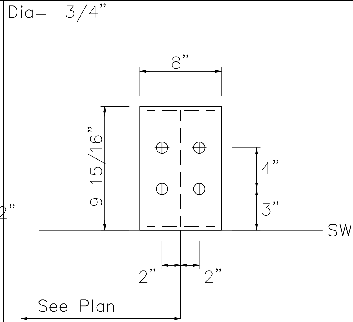
DETAIL D
