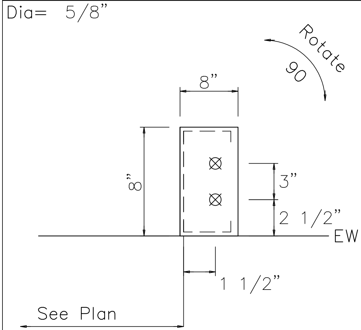
DETAIL A
