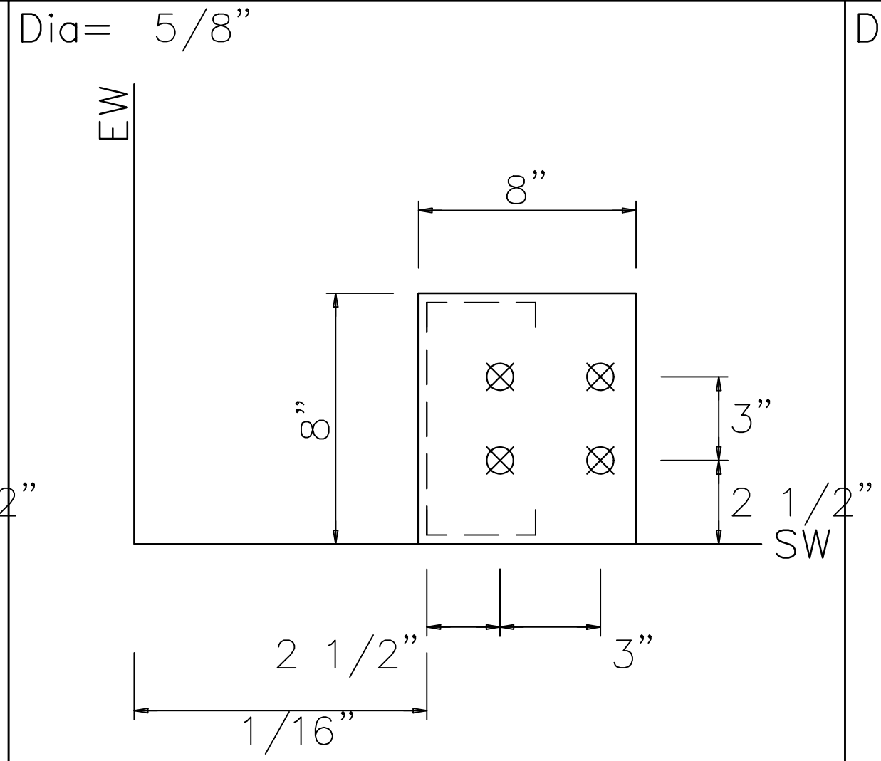
DETAIL C
