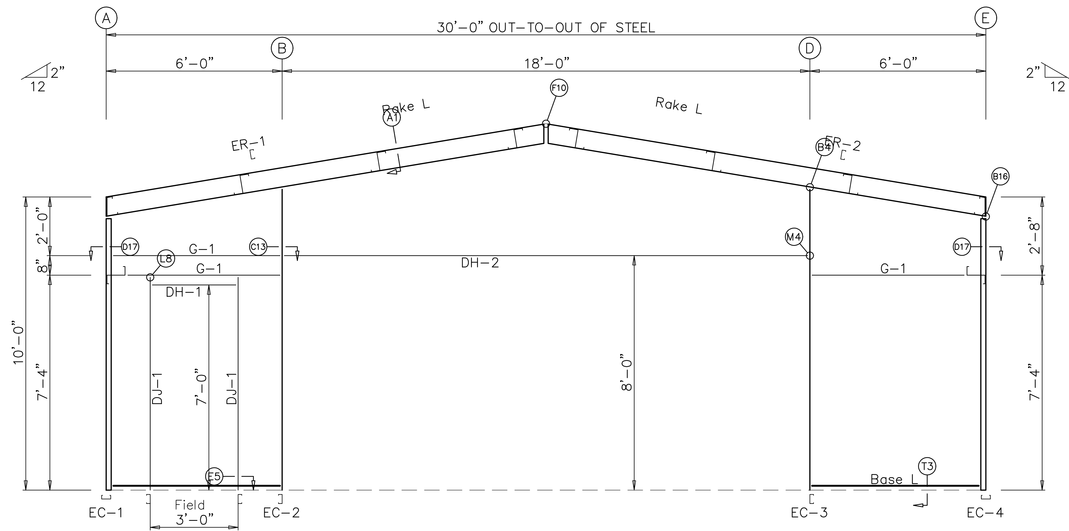
ENDWALL FRAMING: FRAME LINE 1
