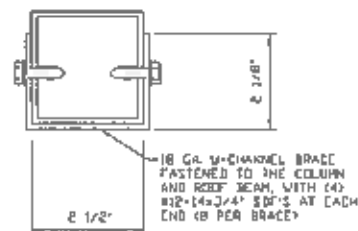
BOX EAVE RAFTER COLUMN CONNECTION DETAIL FOR HEIGHTS ≤ 10'-0" SCALE: NTS
