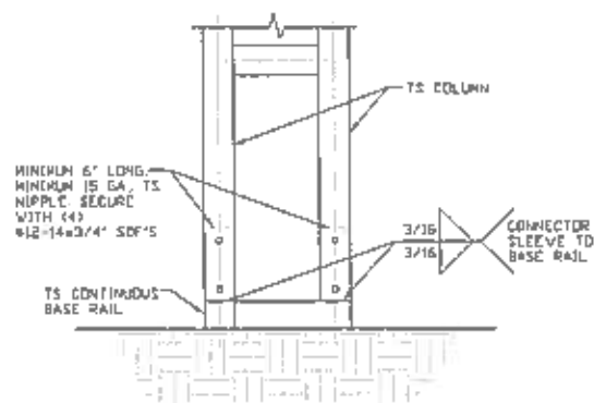
RAFTER COLUMN/BASE RAIL CONNECTION DETAIL SCALE: NTS
