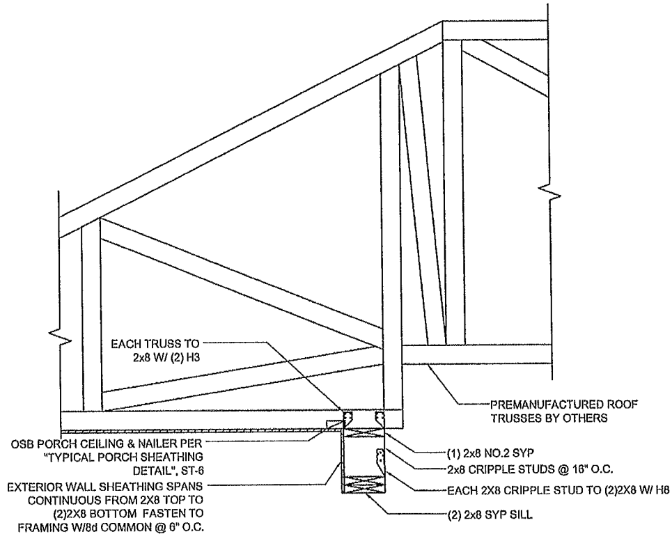
B1 SECTION THRU SUSPENDED HEADER ST-6
