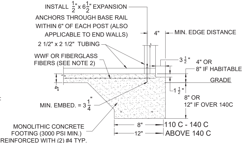
3A CONCRETE MONOLITHIC SLAB BASE RAIL ANCHORAGE SCALE: NTS
