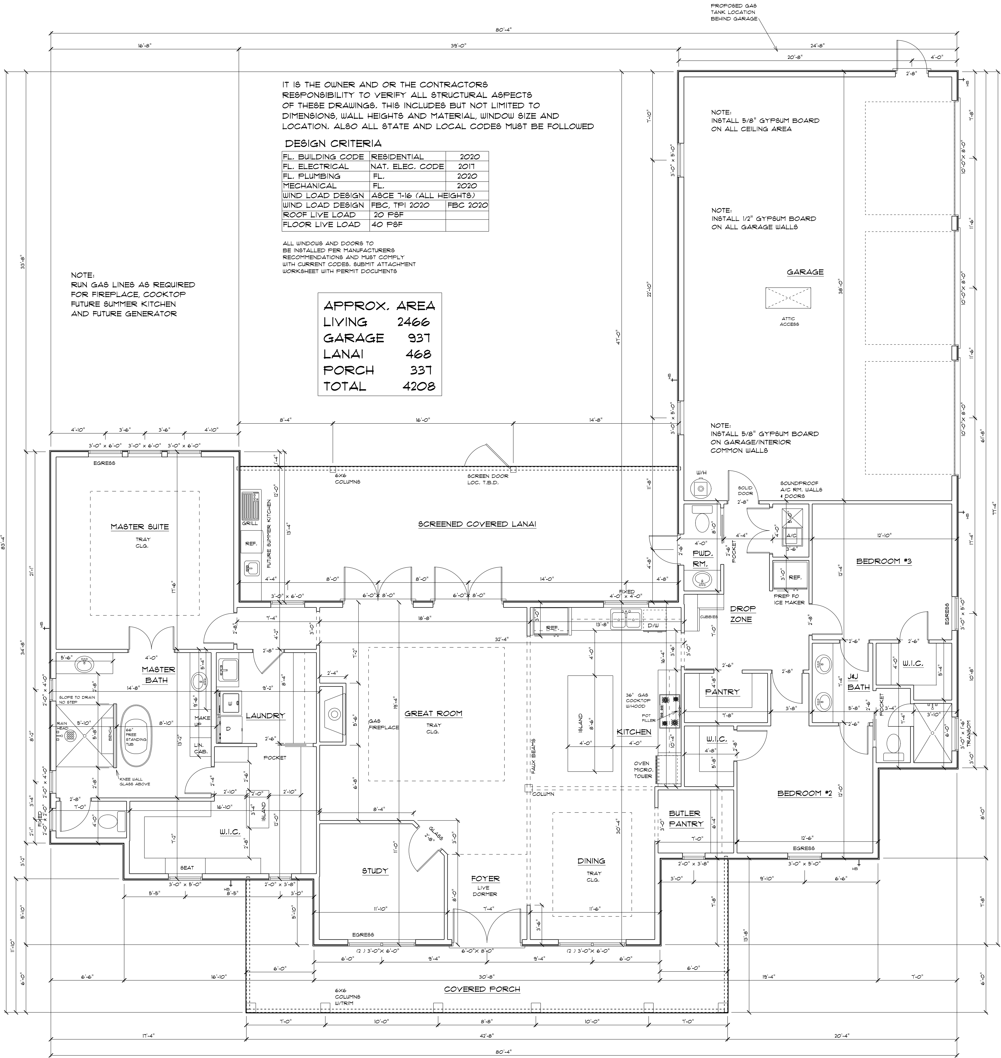
MAIN FLOOR PLAN
