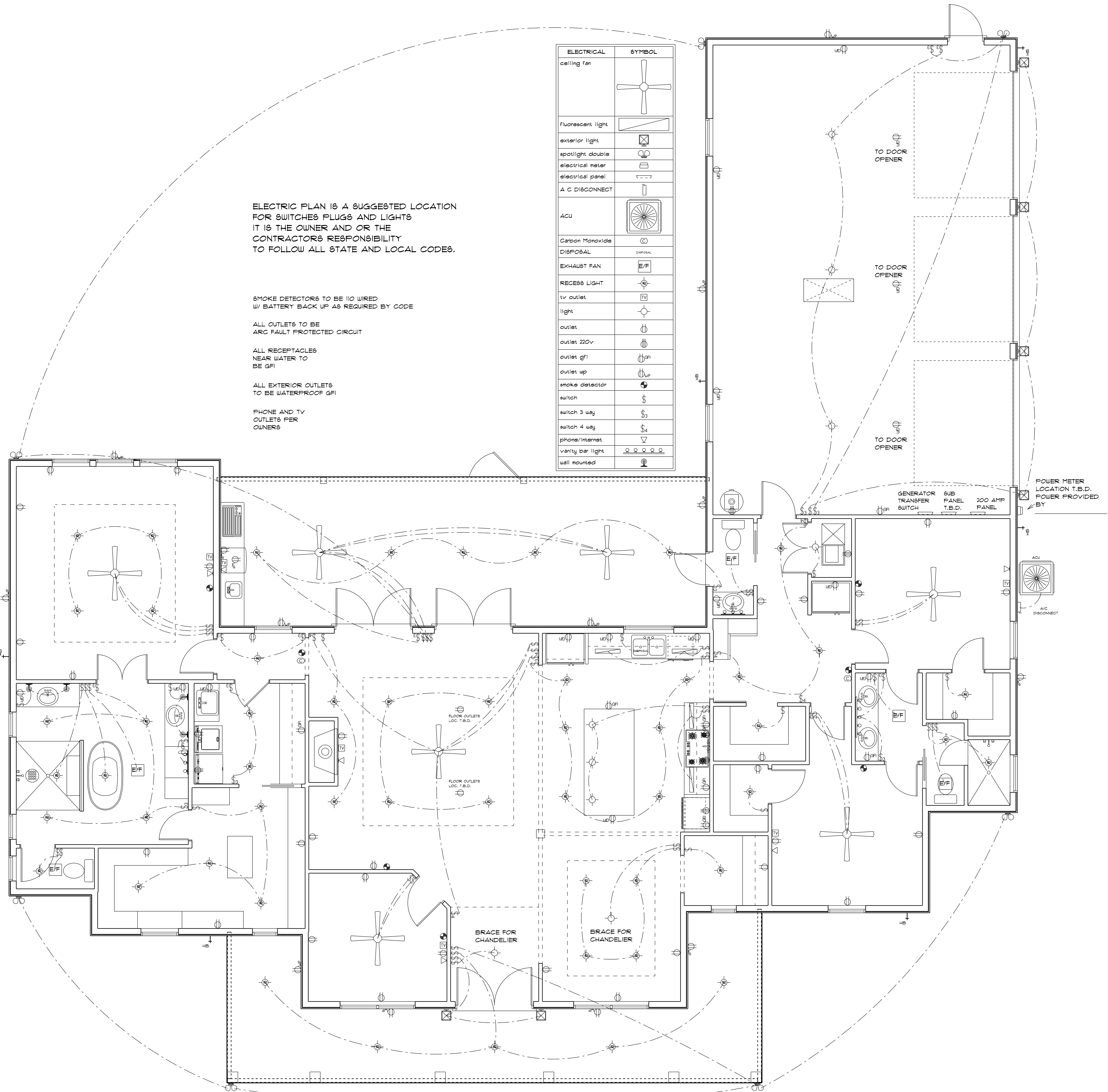
ELECTRICAL PLAN
